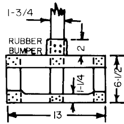
Fig. 15. Piston Rod Handle Made of 3/4 \times 1\text{-}3/4 -in. Boards.
