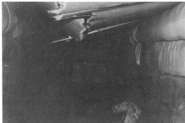
Fig. D.4. Post-blast interior of an Above-ground, Door-Covered Shelter that survived 1-kiloton blast effects at the 5.8-psi overpressure range. The shelter walls were made of bedsheets containing earth, as described in Appendix A.
