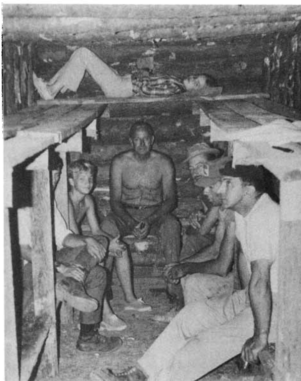
Fig. 14.2. Benches with overhead bunks in a skillfully designed Small-Pole Shelter of Russian design. Three rural families in a wooded area of Tennessee built this expedient blast shelter in 48 hours, including the time spent felling trees and making furnishings.
