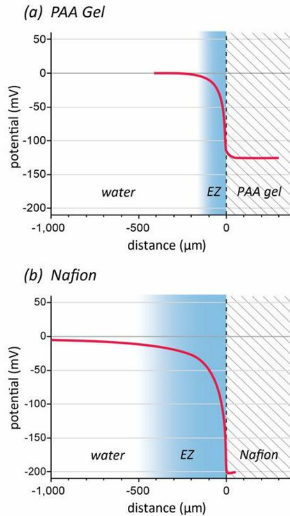
Fig. 4.7 Electrical potentials measured near a polyacrylic acid gel (a), and a Nafion sheet (b). The zone of negativity correlates with the width of the EZ, which differs in the two cases.
