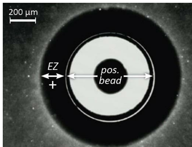
Fig. 4.17 EZs surround both negatively and positively charged beads.
