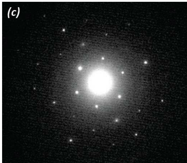
Fig. 4.11 Protein-encapsulated water. 14 Encapsulation produces spheres (a) seen in the scanning electron microscope, and geometric figures (b) seen in the transmission electron microscope. Diffraction pattern (c) obtained from geometric figure shows hexagonal order.
