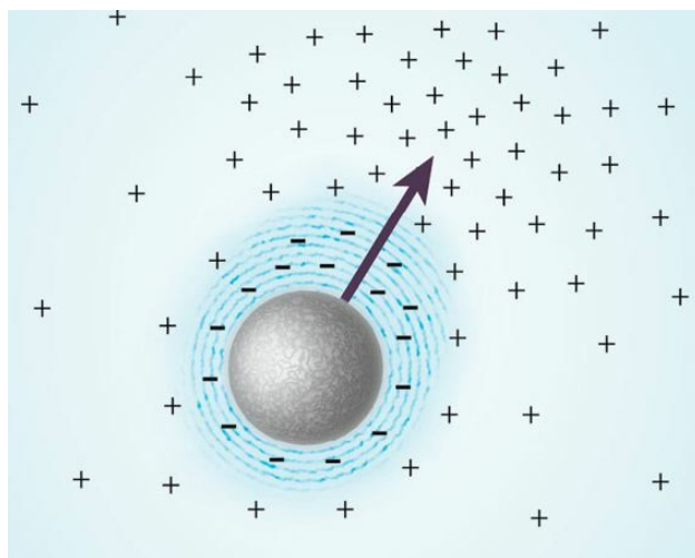
Fig. 9.7 More intense incident energy (from upper right) should yield an asymmetric charge distribution. This asymmetry gives rise to a net electrostatic force, moving the object and its EZ in the direction of maximum incident energy.
