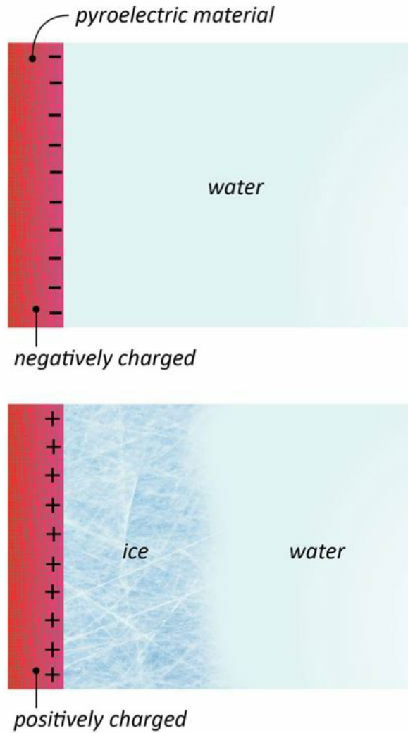
Fig. 17.6 Pyroelectric experiments. Negative charge retards ice formation, while positive charge promotes ice formation.
