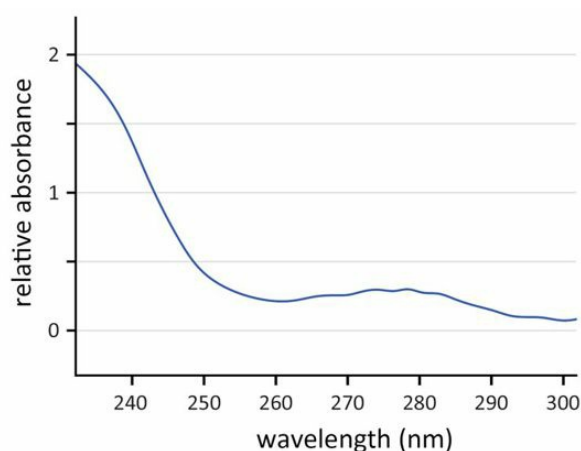
Fig. 10.9 UV-Vis spectrometer recording of 50:50 mixture of HCl and water. A peak appears at 278 nm.
