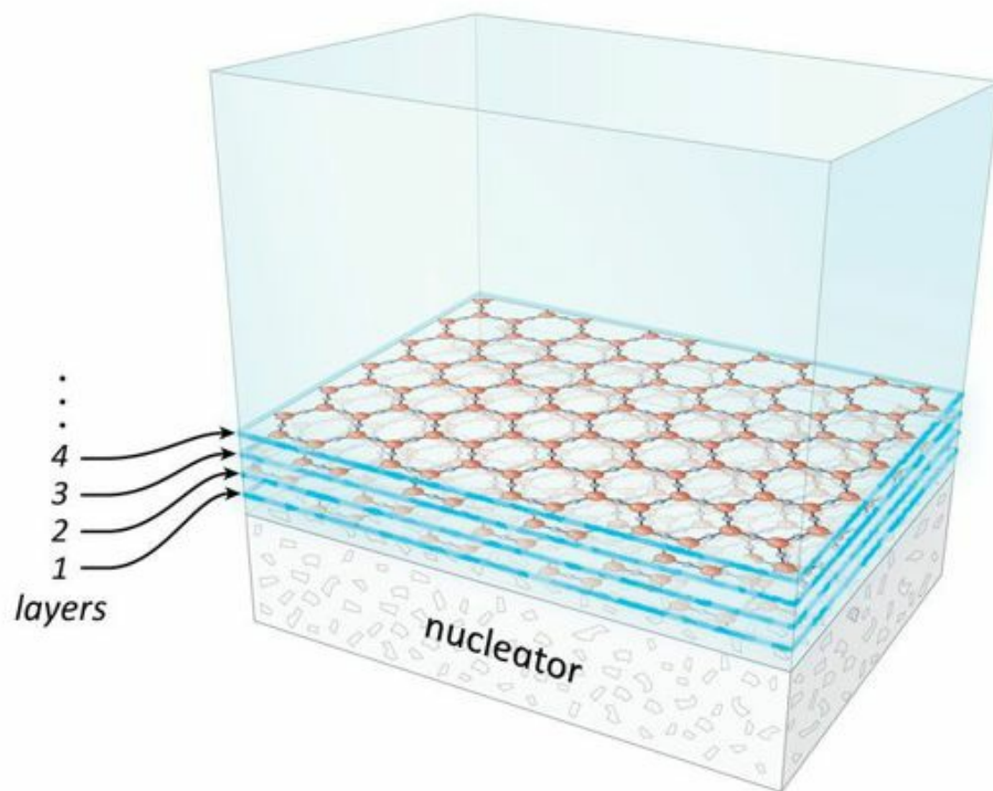
Fig. 4.15 Buildup of honeycomb planes from bulk water. Hydrophilic surface nucleates EZ growth, which progresses layer by layer.
