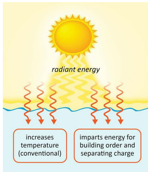
Fig. 7.13 Energetic pathways within water. The conventional pathway is heating; the newly revealed pathway is the creation of deliverable potential energy. This latter pathway may be the generic first step in photosynthesis.
