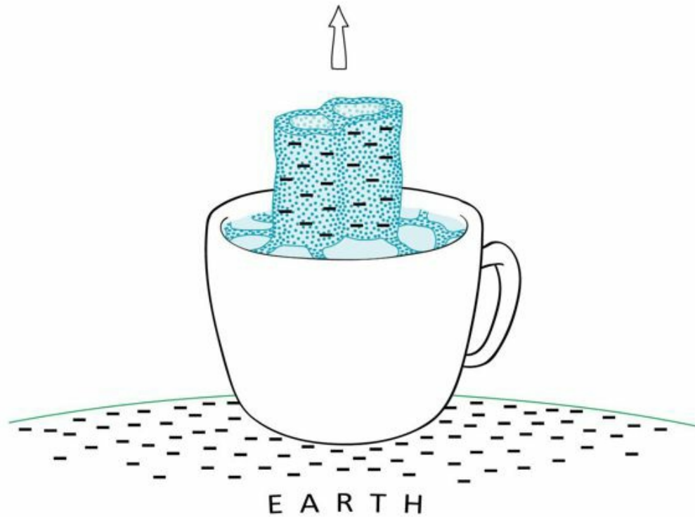
Fig. 15.13 Negatively charged vesicles are repelled from the surface of the earth.
