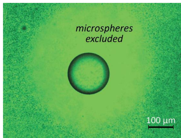
Fig. 3.7 Microspheres excluded from the vicinity of a charged gel bead, as seen in an optical microscope. (Color arises because of microscope filter.) We positioned the bead on a glass surface and added the microsphere suspension. The EZ grew with time to the extent shown.
