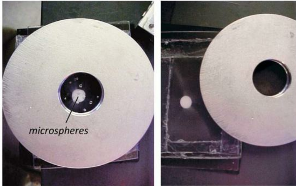
Fig. 9.10 Light-induced attraction of microspheres. Light shines through a hole in an aluminum mask. After some time, microspheres in the chamber beneath the mask gather at the center of the hole.
