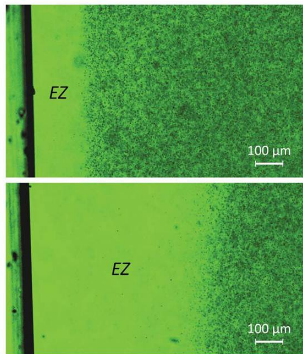
Fig. 6.1 Exclusion zone adjacent to Nafion. Top: control. Bottom: following several minutes of exposure to light.
