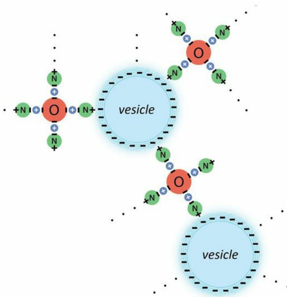
Fig. 15.18 Vesicles might loosely link oxygen-nitrogen complexes to form a continuous structure.
