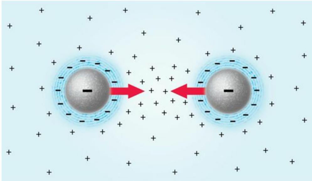
Fig. 18.5 Mediated attraction of likes by unlikes.
