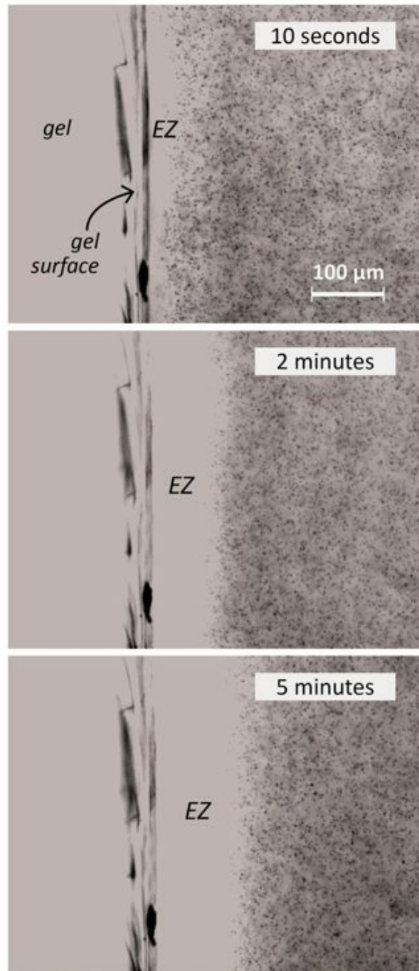
Fig. 3.4 Microsphere-exclusion zone (EZ) next to a gel surface. The zone grows with time and then remains relatively stable after about five minutes.
