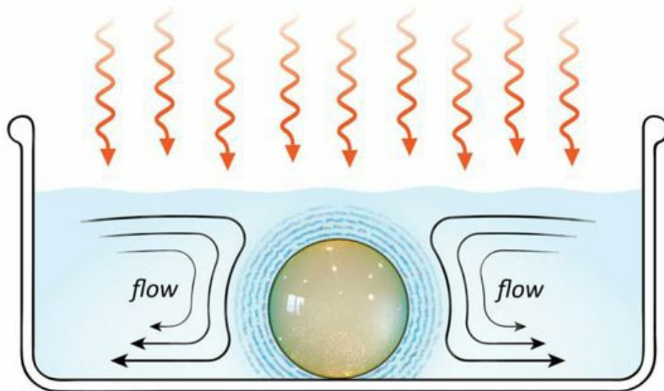
Fig. 12.14 Sustained flow pathways around a hydrophilic sphere.
