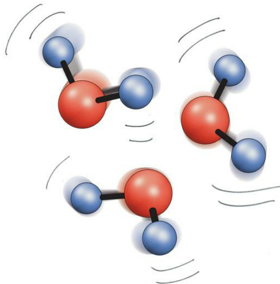
Fig. 2.2 Interaction among water molecules. The nature of the interaction is not well understood.
