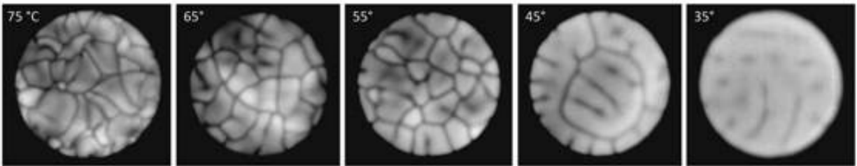
Fig. 15.4 Infrared camera recordings of water surface patterns at a series of temperatures.
