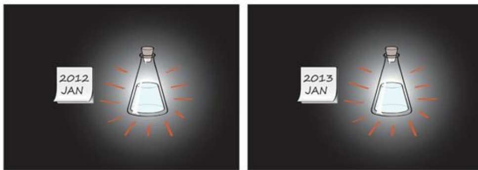
Fig. 7.5 Aqueous solutions can produce practically eternal light output.
