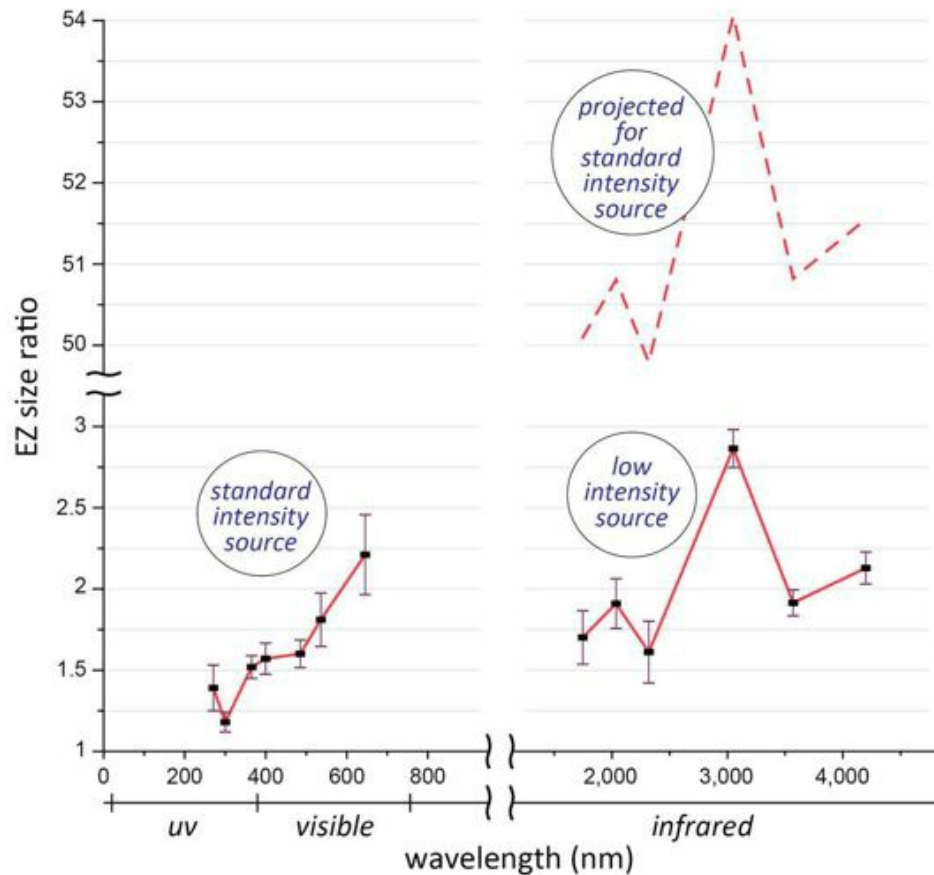
Fig. 6.2 Effect of incident light wavelength on EZ growth. EZ size ratio (ordinate) refers to EZ size at the end of a five-minute exposure to light, relative to its size before adding light. For technical reasons, data on the right side were obtained with low-intensity light sources. Intensities similar to those used for obtaining the data on the left would have elevated the graph, as estimated by the dashed curve above.
