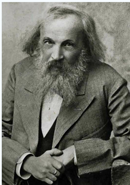
Dmitry Mendeleev 1834–1907
