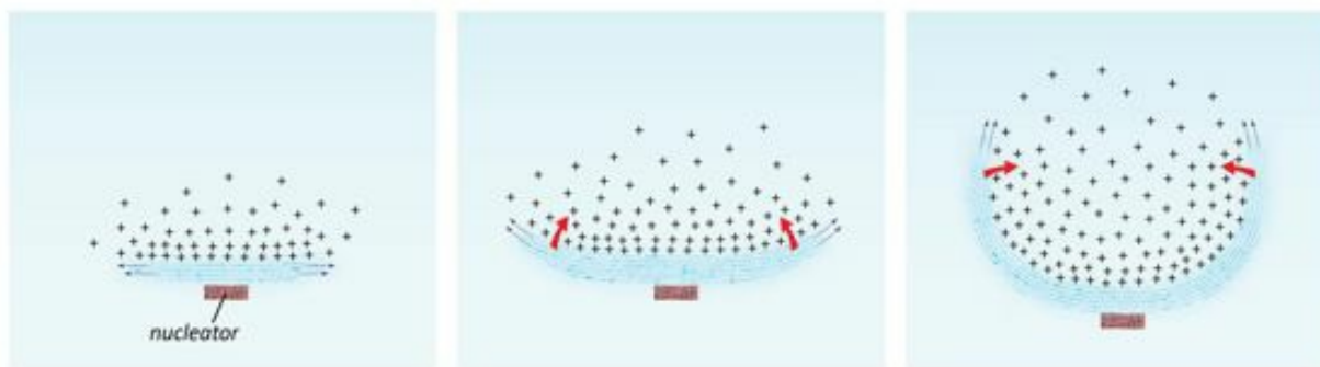
Fig. 14.1 Stages of vesicle formation. Left: EZ grows layer by layer, and also laterally (arrows). Protons build positive charge beyond. Middle: EZ deflects because of attraction to positive charge. Red arrows indicate direction of deflection. Right: continued deflection creates vesicle.
