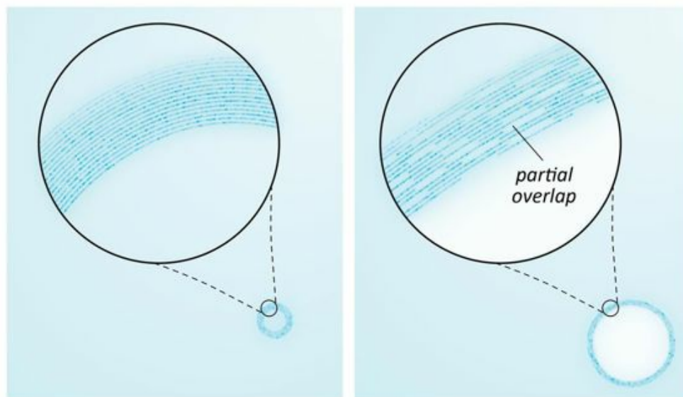
Fig. 14.3 Vesicle expansion. To accommodate the pressure-induced expansion, EZ layers slide over one another to partially overlap.
