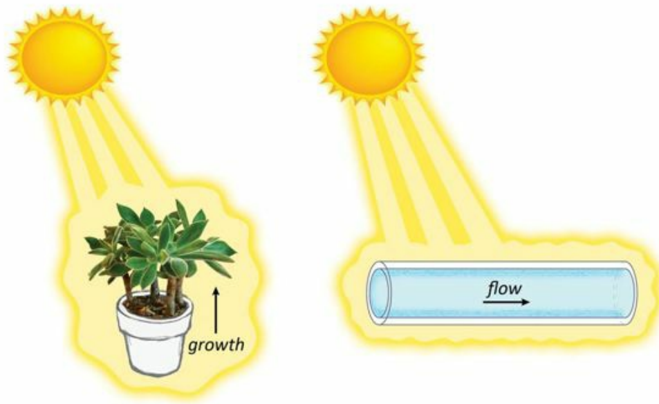
Fig. 9.5 Radiant energy produces work in plants and in water; the two processes are conceptually similar. By processing input energy, both operate out of equilibrium.
