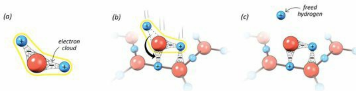
Fig. 6.8 Electron cloud shifts as water bonds to lattice. The shift frees the dangling proton.
