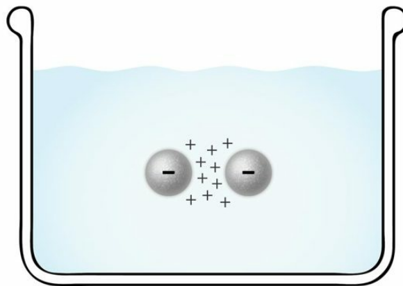
Fig. 8.1 Negatively charged particles may attract if enough positive charges lie in between.
