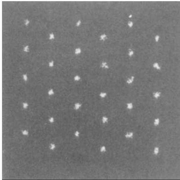
Fig. 8.3 Eventual distribution of latex particles: 0.4 \mu\text{m} in diameter, 2% concentration in aqueous suspension. 3
