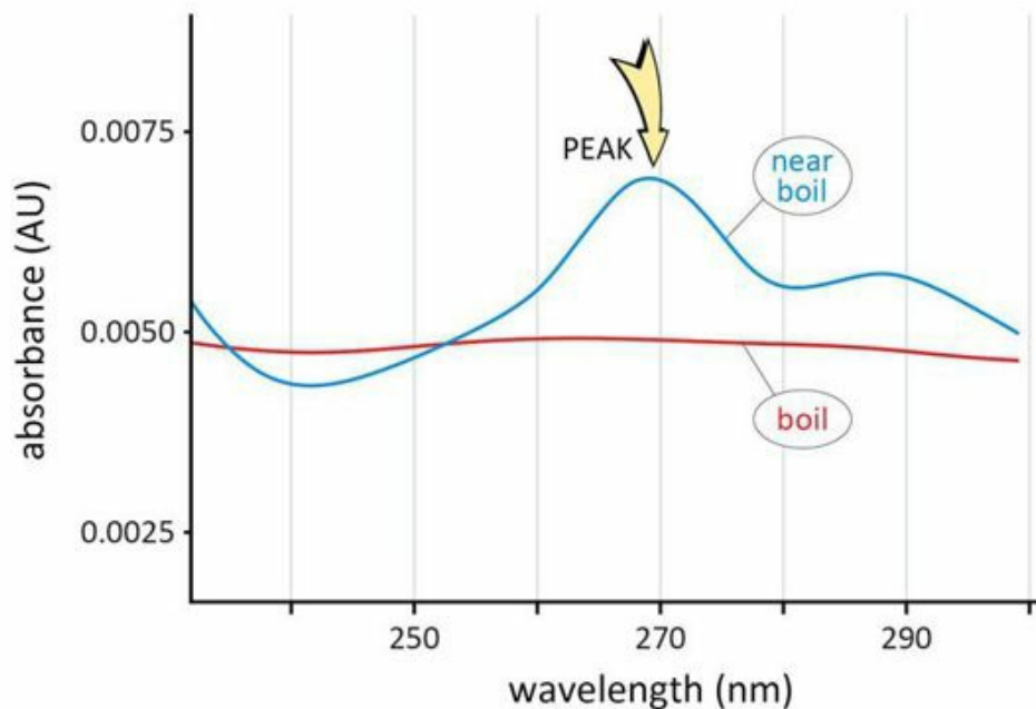
Fig. 13.9 Absorption spectra of water previously heated to just below boiling
