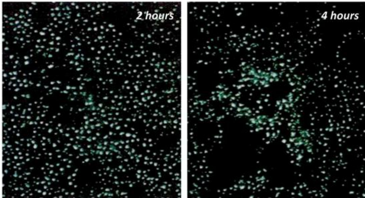
Fig. 8.4 Microspheres draw together over time, leaving large voids that contain no microspheres. Frame width: 10 \mu\text{m} . 4
