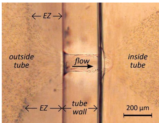
Fig. 7.11 Inward flow produced by hole punched in the wall of a Nafion tube. View is from top of chamber. The inwardly flowing microsphere suspension moves towards the two open ends of the tube.
