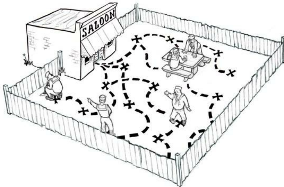
Fig. 11.1 Random walks will eventually lead to a statistically uniform distribution spread out over a defined space.
