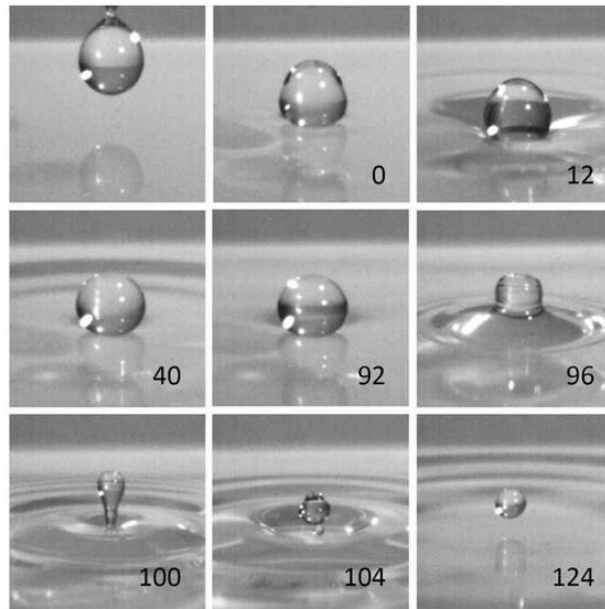
Fig. 16.17 Several stages of water droplet dissolution in water. 8 Numbers indicate time from when the droplet lands, in milliseconds.
