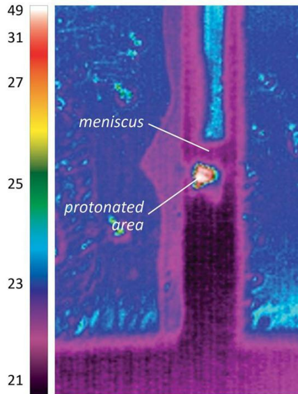
Fig. 16.14 Infrared image of water rising in a square capillary tube. Note the hot spot just beneath the meniscus. Scale in °C.
