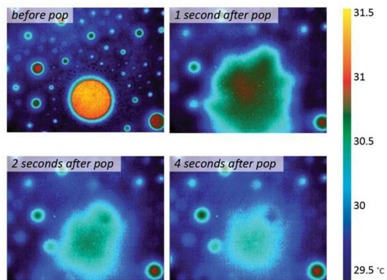
Fig. 14.7 Bubble collapse. Similar to Figure 14.6, except that one bubble pops spontaneously. Note the dispersal of the zone of high radiant energy. Scale in °C.
