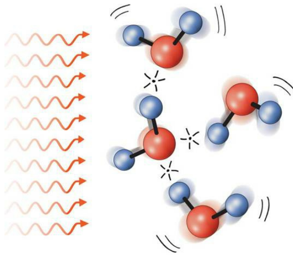
Fig. 6.6 Input energy may dissociate water molecules from one another.
