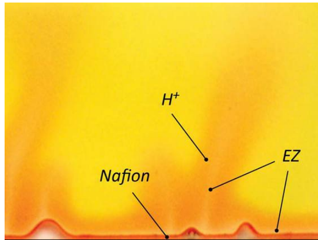
Fig. 5.6 Similar to Figure 5.3 , taken at a lower magnification and later time. Note zones of low pH (red) surrounding each vertical EZ projection.
