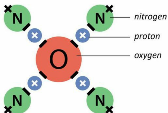
Fig. 15.17 Simplified schematic of possible gas linkages (not to scale). Protons might link electronegative sites on oxygen and nitrogen, creating stoichiometric linkages such as the one shown. The actual number of molecules would be larger.
