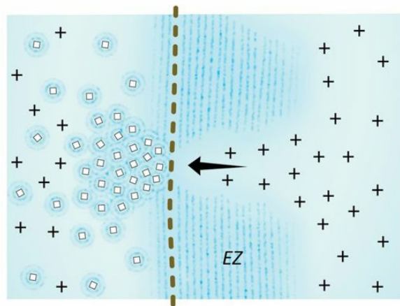
Fig. 11.8 EZ clustering against membrane draws hydronium ions leftward.
