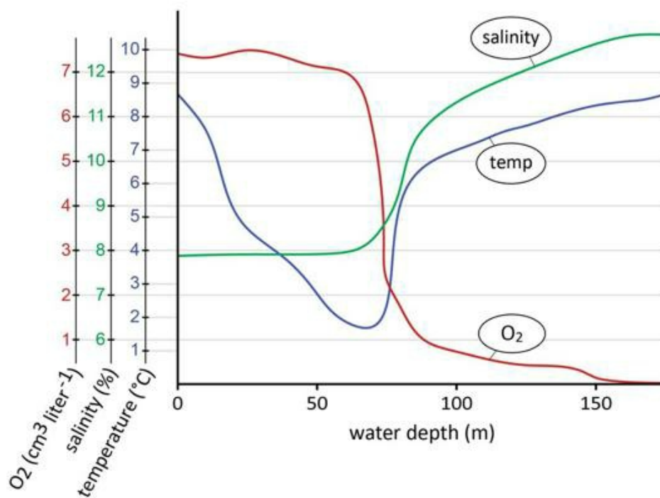
Fig. 16.5 Vertical profiles in the ocean. 2 Temperature, dissolved oxygen, and salinity profiles, measured at Baltic Sea station, 26 May, 1979.
