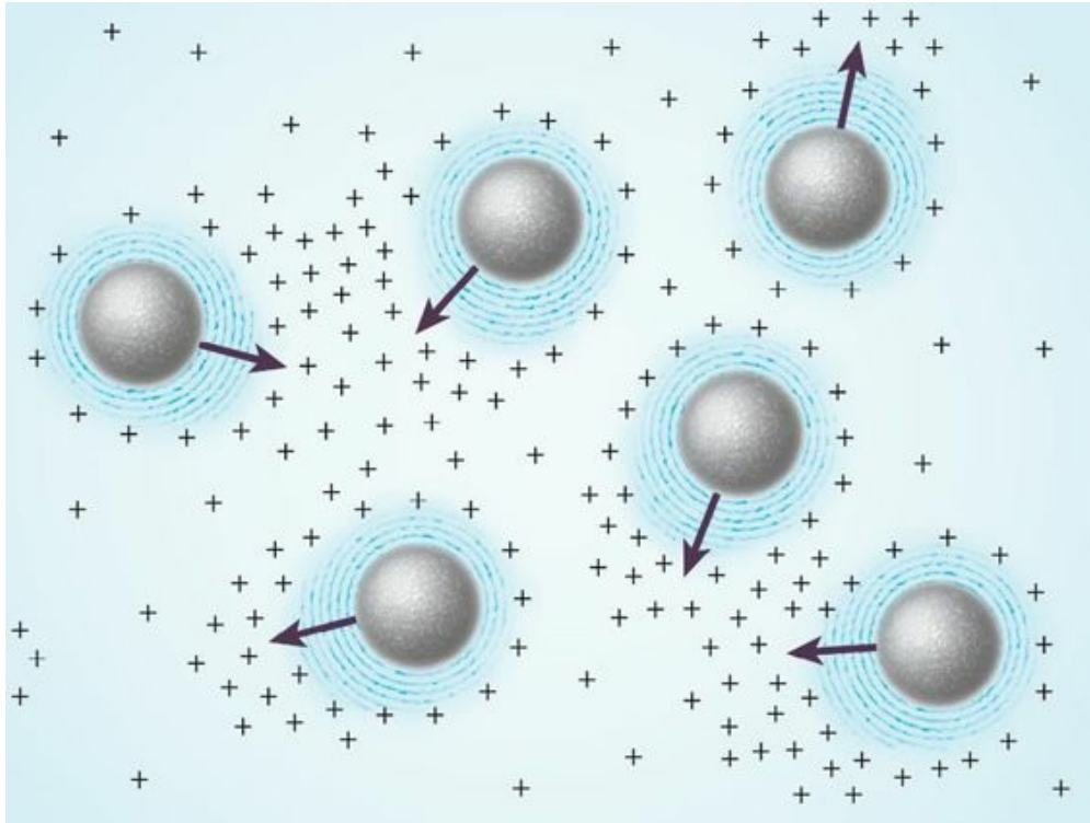
Fig. 9.14 Charge distributions surrounding microspheres in suspension. Arrows denote anticipated directions of movement of negative particles toward positive-charge maxima. Directions will continually change as particles move.
