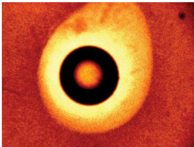
Fig. 9.8 Asymmetric exclusion zone around a gel bead, resulting from incident light coming from top right.
