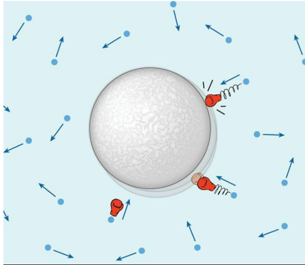
Fig. 9.2 Origin of Brownian motion according to Einstein. Water molecules continually bombard the particle with mechanical energy. That energy produces movement.
