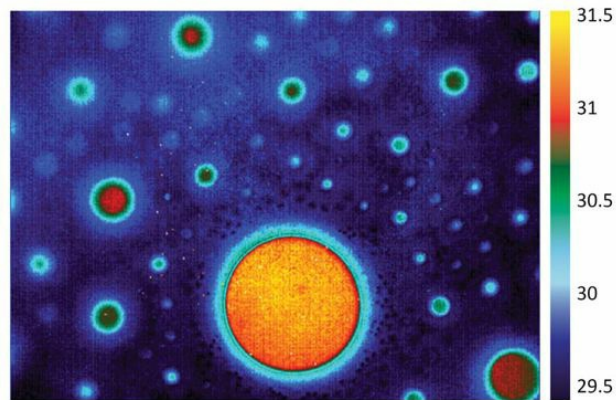
Fig. 13.10 Surface bubbles tend towards ordered arrangements. Bubbles were created by pumping air into an aqueous detergent (TWEEN 20) solution. Scale in °C.
