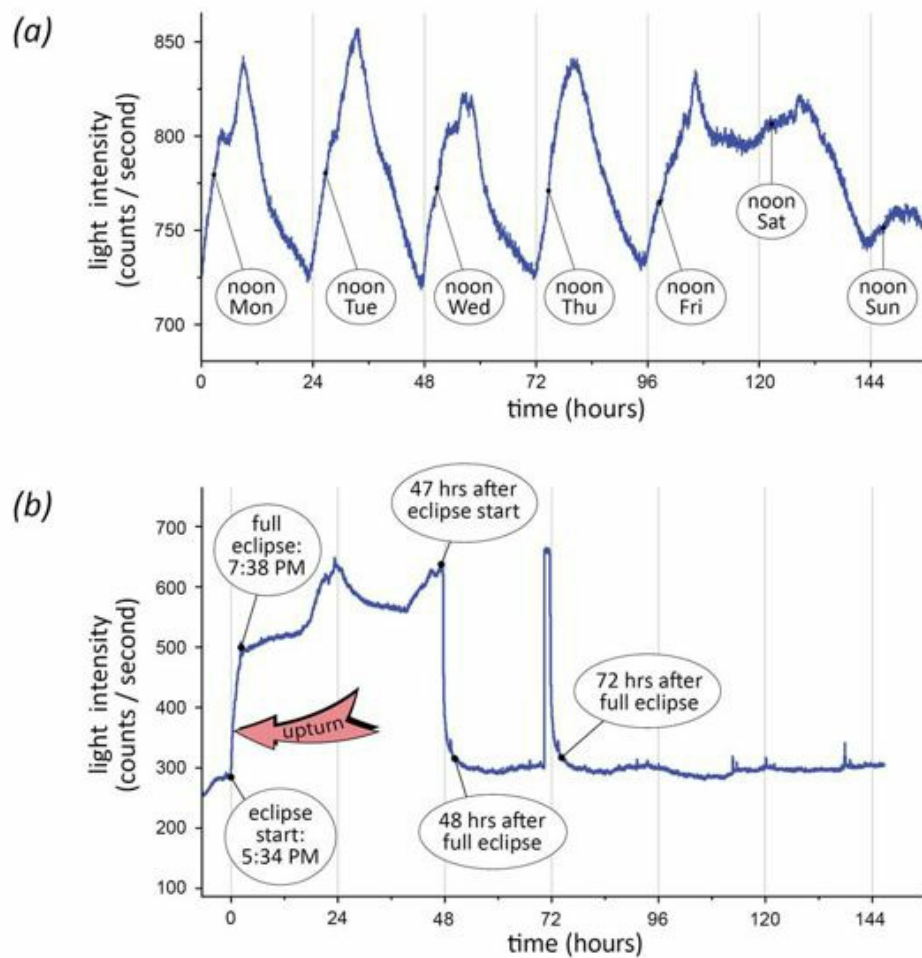
Fig. 7.3 (a) Light emission recorded from water containing bicarbonate ions and enhanced by dissolved luminol. Note the periodic intensity variation. (b) Similar to (a) but recorded during an eclipse of the moon.
