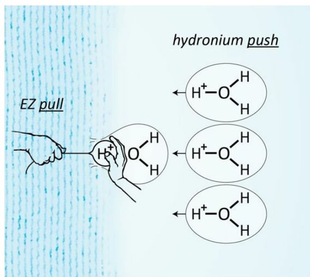
Fig. 17.12 Forces exerted on a near-EZ hydronium ion. EZ negativity pulls on the proton (left) while many bulk-water hydronium ions push (right), eventually dislodging it from the parent water molecule. Once dislodged, the proton can easily penetrate into the negative EZ.
