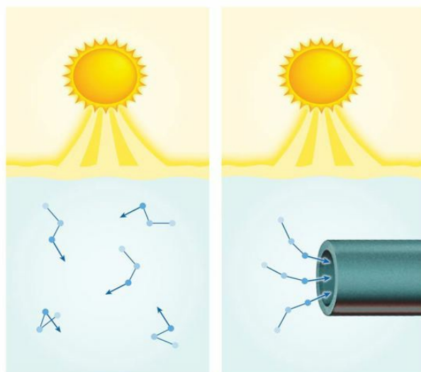
Fig. 9.6 Incident energy generates motions, which can be random or coordinated, in the absence (left), or the presence (right) of a director.
