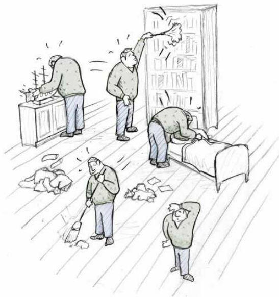
Fig. 6.9 Building order requires considerable energy input. Creating the original mess requires much less energy.
