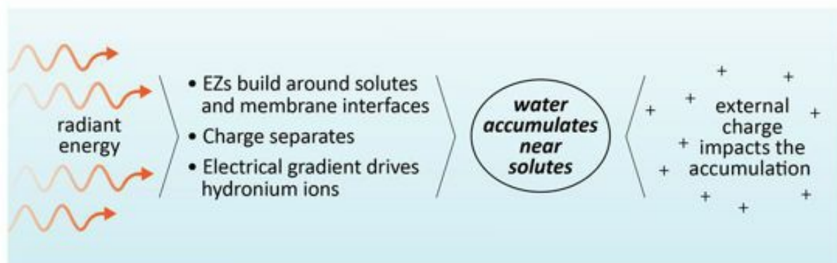
Fig. 11.9 Summary of diffusion and osmosis mechanisms, illustrating common features.
