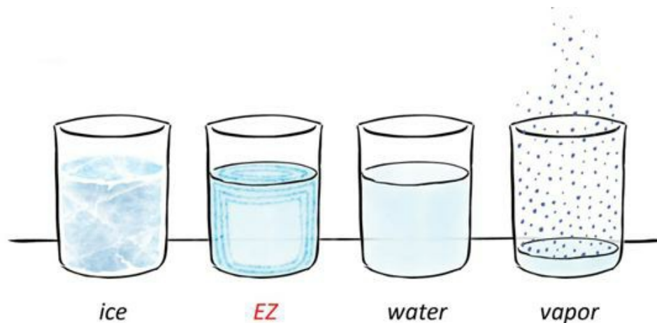
Fig. 18.2 Water's four phases.
