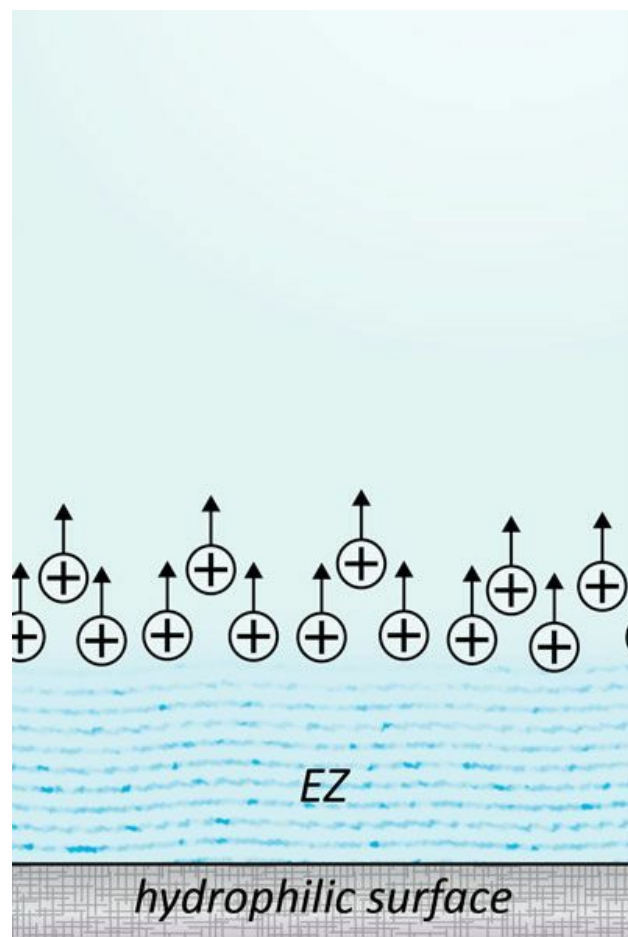
Fig. 5.2 Protons generated at the leading edge of growing exclusion zone.
