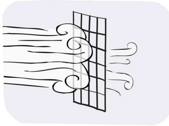
Fig. 15.15 Ordinary window screens reduce moist air flow more than anticipated.
