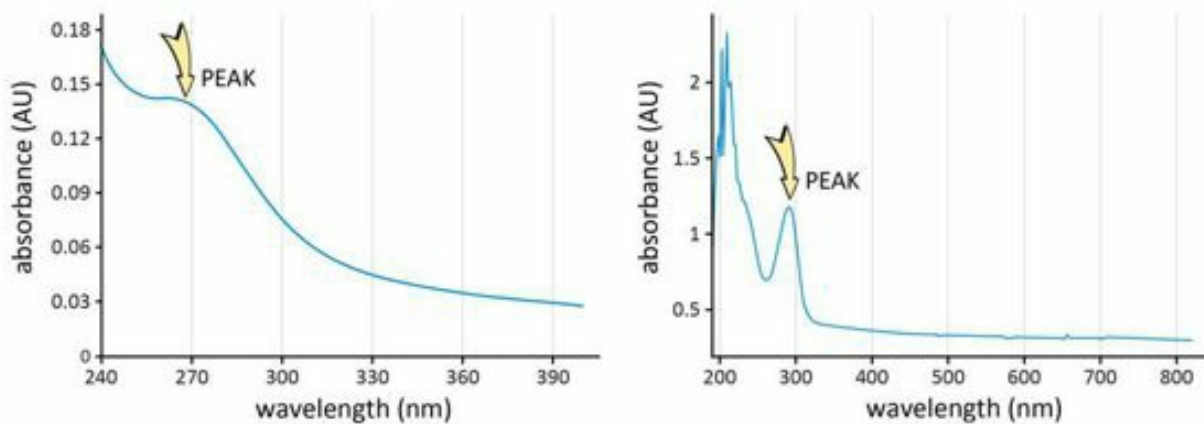
Fig. 13.7 UV-Vis spectra obtained from raindrops collected from two different rainfalls. A peak near 270 nm is evident on the characteristic descending curves.
