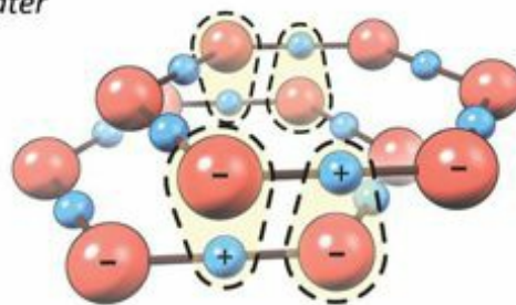
Fig. 12.5 The effect of pressure on ice. The pressure squeezes out protons, which converts the ice to EZ water.
