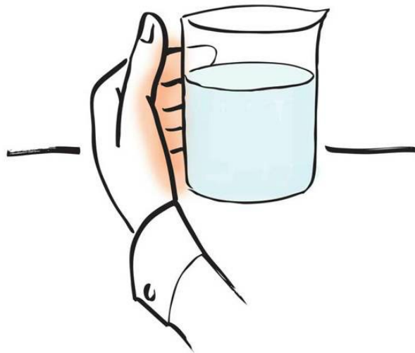
Fig. 10.7 Your hand senses the amount of radiant energy coming from the water.
