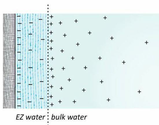
Fig. 5.10 Diagrammatic representation of the EZ water battery. Hydrophilic surface at left. The separated charges are deliverable.
