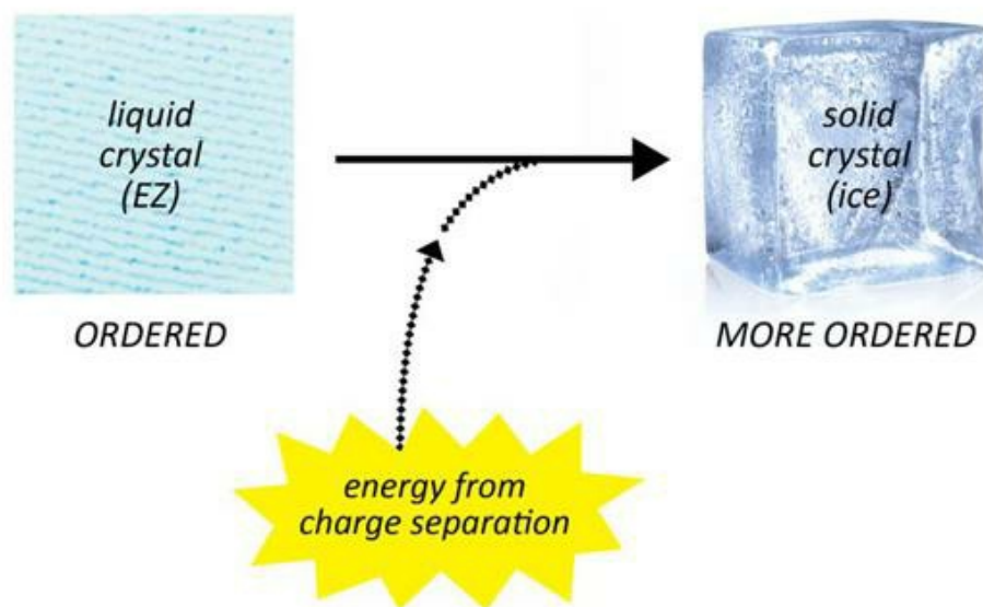
Fig. 17.2 Energetic aspects of the transition from EZ water to ice. The required energy comes from separated protons.
