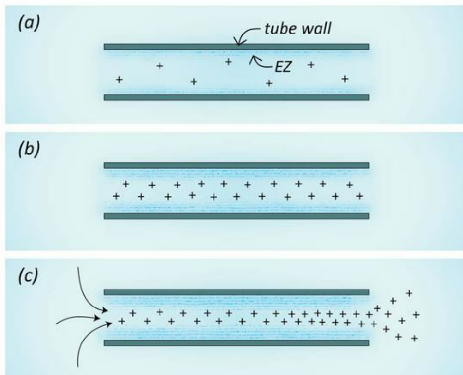
Fig. 7.10 Mechanism of intratubular flow. The key element is the hydronium-ion buildup in the tube core, and its escape to the water outside.
