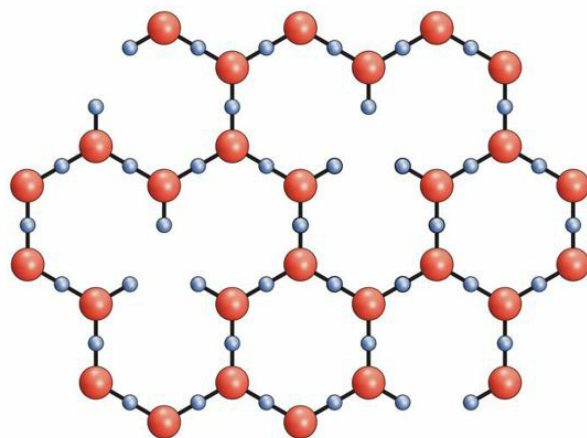
Fig. 4.16 Diminishing planar charge. The example shows how removal of oxygen atoms from the hexagonal lattice can occur without impairing structural integrity.
