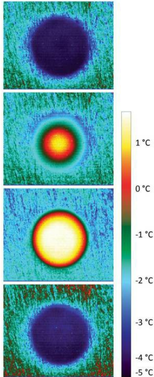
Fig. 17.10 Infrared emission from a water droplet during freezing on a cold surface. The droplet emits a brief flash of infrared light as it freezes (top to bottom). Frame times in seconds:
