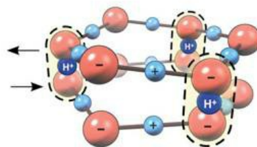
(c) layers align to form ice
