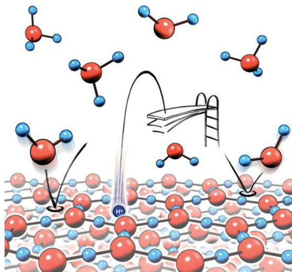
Fig. 17.11 Only protons are small enough to penetrate into the EZ lattice.
