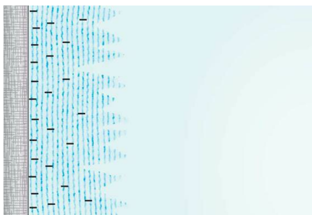
Fig. 6.10 Jagged outer reaches of the exclusion zone. Hydronium ions penetrate the valleys between the mountain peaks because of attraction to negative charges.
