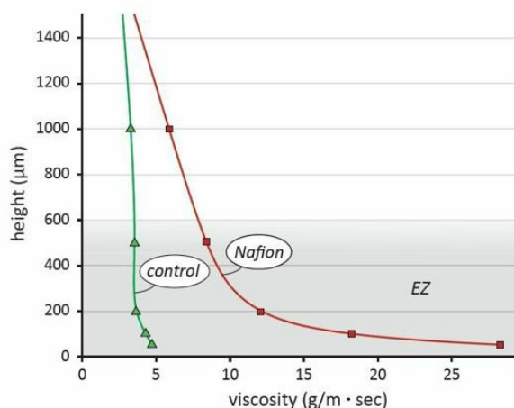
Fig. 3.17 Viscous character of the EZ (shaded). We measured viscosity in water at various heights above a Nafion surface (red curve). Control (green curve) was obtained with a surface exhibiting little or no exclusion zone.
