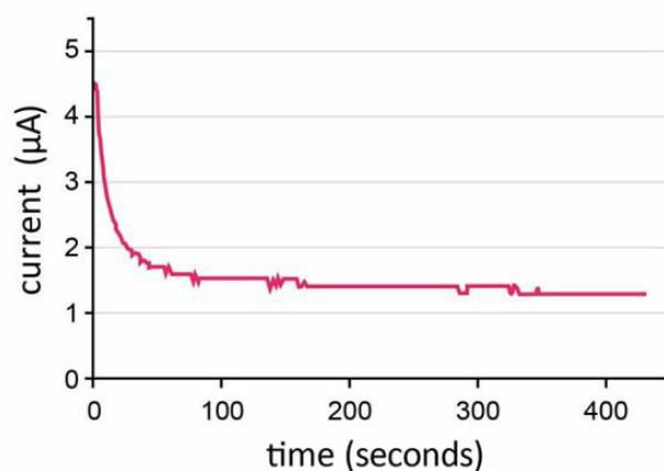
Fig. 5.7 Current flow from separated charges in EZ and the water beyond. Current begins flowing immediately after immersing electrodes, maintaining a nonzero plateau value for an extended period of time.
