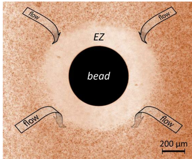
Fig. 7.12 A gel bead (top view) positioned in a chamber containing water and microspheres generates a consistent flow pattern around the bead.
