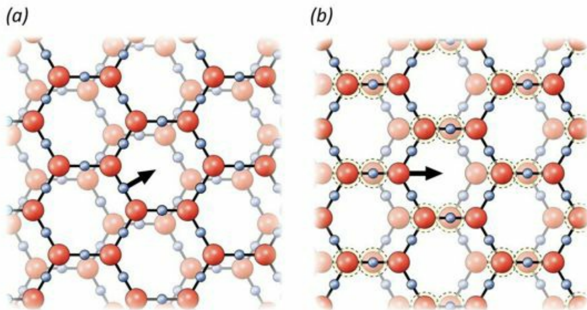
Fig. 4.13 Possible plane-stacking arrangements involving linear shifts. Only the shift shown in the right panel yields a stable structure with overlapping opposite charges.
