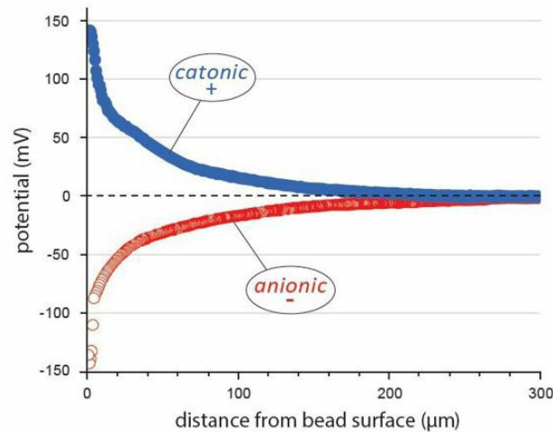
Fig. 4.18 Electrical potentials recorded next to cationic and anionic beads.
