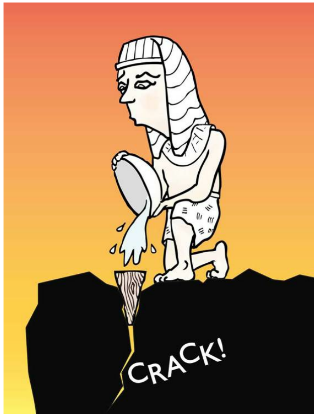
Fig. 12.3 Cracking rocks by exploiting hydration.
