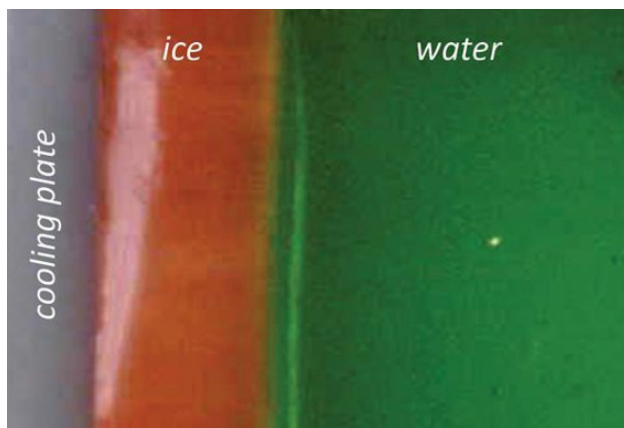
Fig. 17.8 Color of pH-sensitive dye during freezing. Deep orange color indicates low pH and hence abundant protons.
