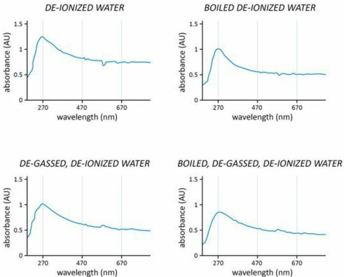
Fig. 17.5 Spectrometer readings obtained from just-melted water. The 270 nm peak is consistently present.
