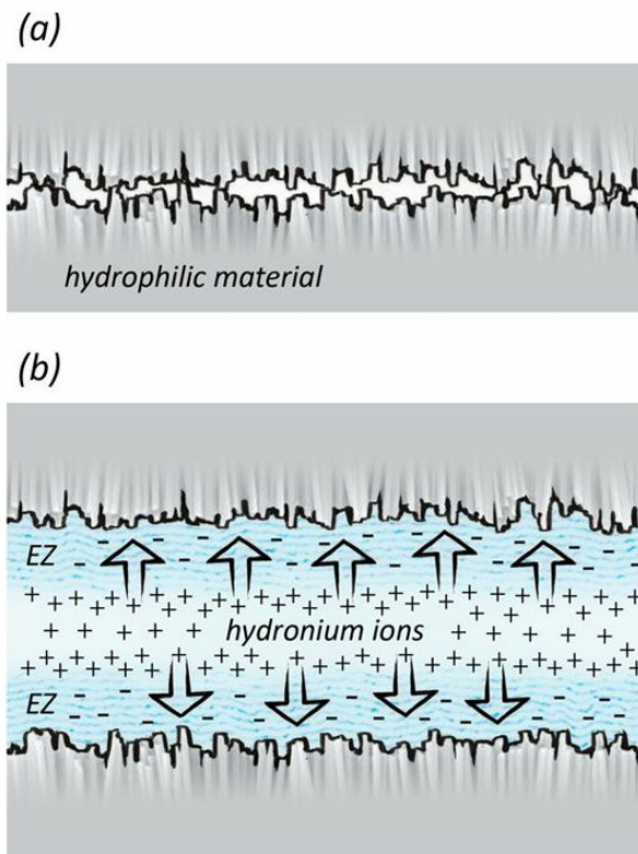
Fig. 12.2 Water and friction. (a) Hydrophilic surfaces may contain friction-generating asperities. (b) With water lodged in between, the
