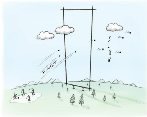
Fig. 15.16 Bug-screen analogy. Even though the boundary is massively large, its presence slows down passing golf balls.
