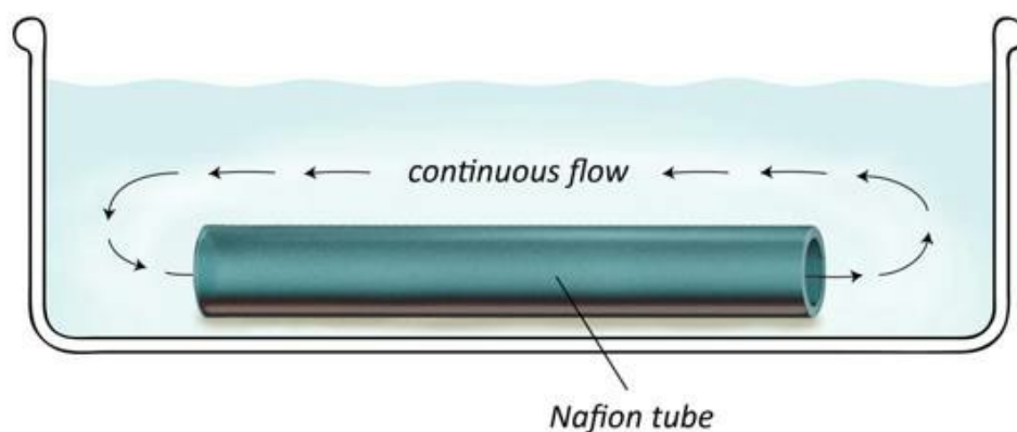
Fig. 7.9 Practically incessant flow occurs through hydrophilic tubes immersed in water.
