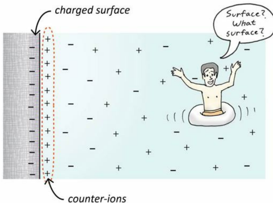
Fig. 3.5 Standard double-layer theory. Charged surface (left) is expected to attract counter-ions of opposite polarity, as shown. Those counter-ions then attract a diffuse cloud of opposite charges, etc. An observer sitting in the water at a site far from the interface should not sense the neutralized surface.
