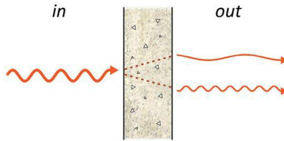
Fig. 10.4 Electromagnetic radiation passing through a complex medium. The character of the radiation may change. Total output energy need not equal input energy if the medium stores energy and uses it to produce work.
