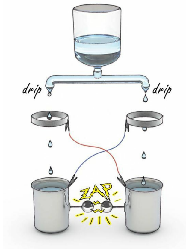
Fig. 1.6 The Kelvin water-dropper demonstration. Rising water levels create a high-voltage discharge. Why does this happen?
