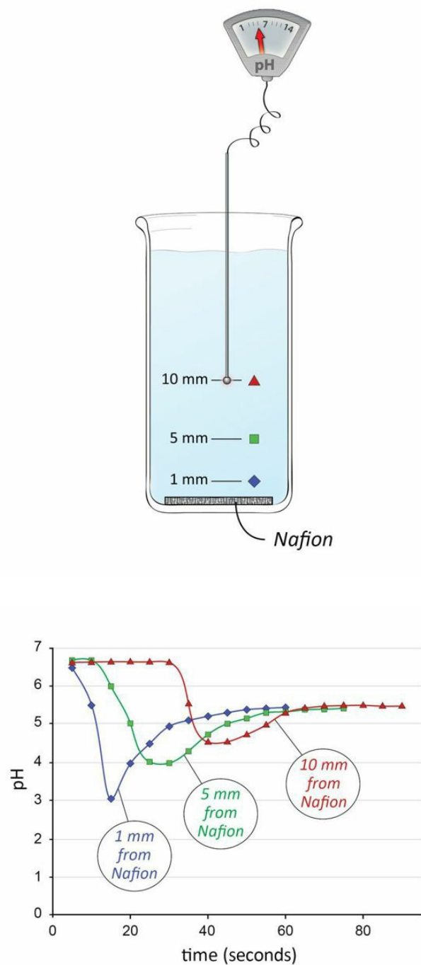
Fig. 5.1 Time course of pH change following the addition of water to a sheet of Nafion. We measured the pH at three points, as indicated. The pattern suggests a progressively rising wave of protons.
