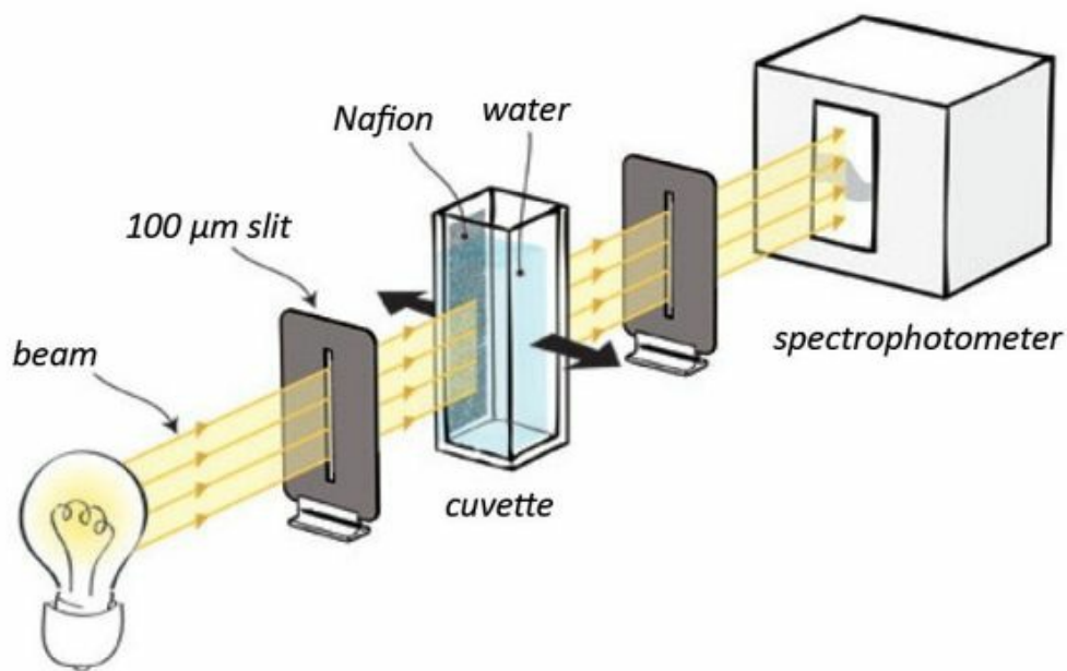
Fig. 3.13a Measurement of light absorption. Moving the cuvette laterally allowed us to interrogate water at various distances from the Nafion surface.
