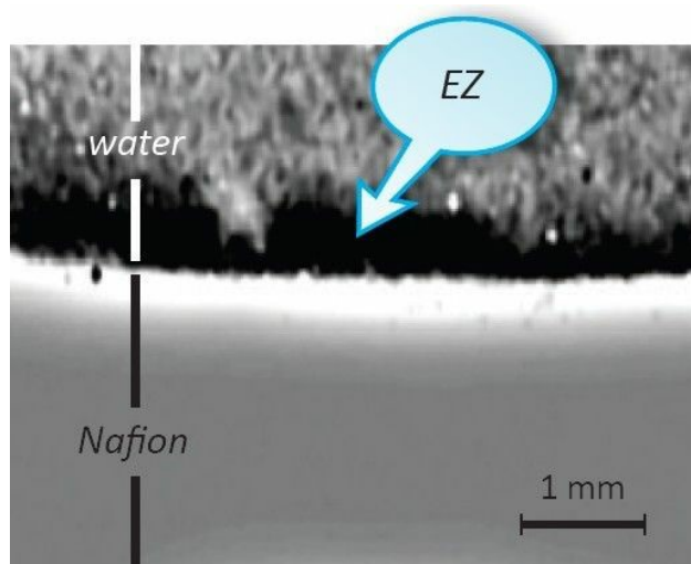
Fig. 3.14 Infrared emission image of Nafion next to water. The sample was equilibrated at room temperature. Black band running horizontally across the middle of the image corresponds to the expected location of the exclusion zone.
