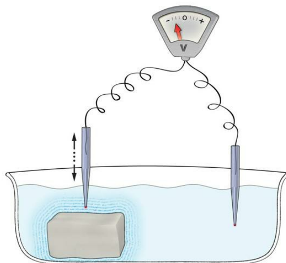
Fig. 4.6 Experimental setup used for measuring the electrical properties of the exclusion zone. Reference electrode at right.
