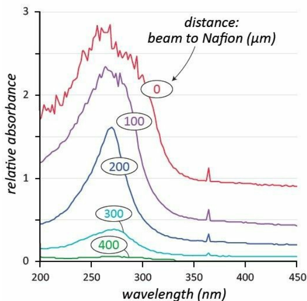
Fig. 3.13b Absorption spectrum measured at various distances from the Nafion-water interface. Decreasing distances range from green to red. Numbers attached to each curve denote actual distances.
