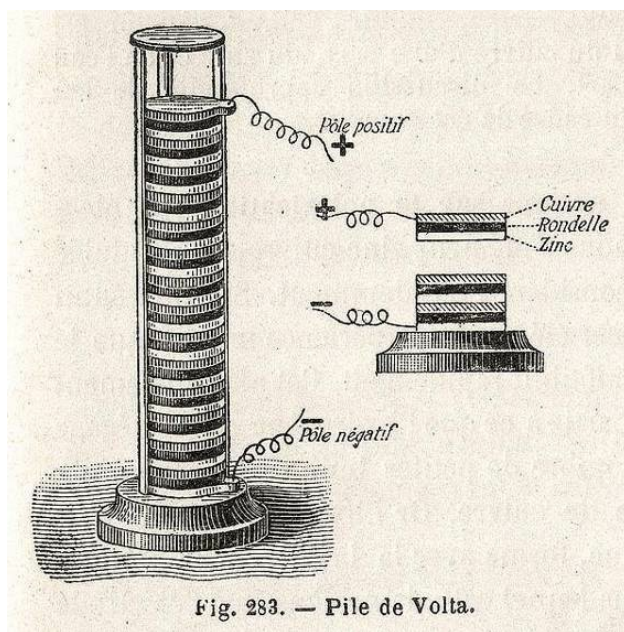
Fig. 12.8 Original pile developed by Volta.
