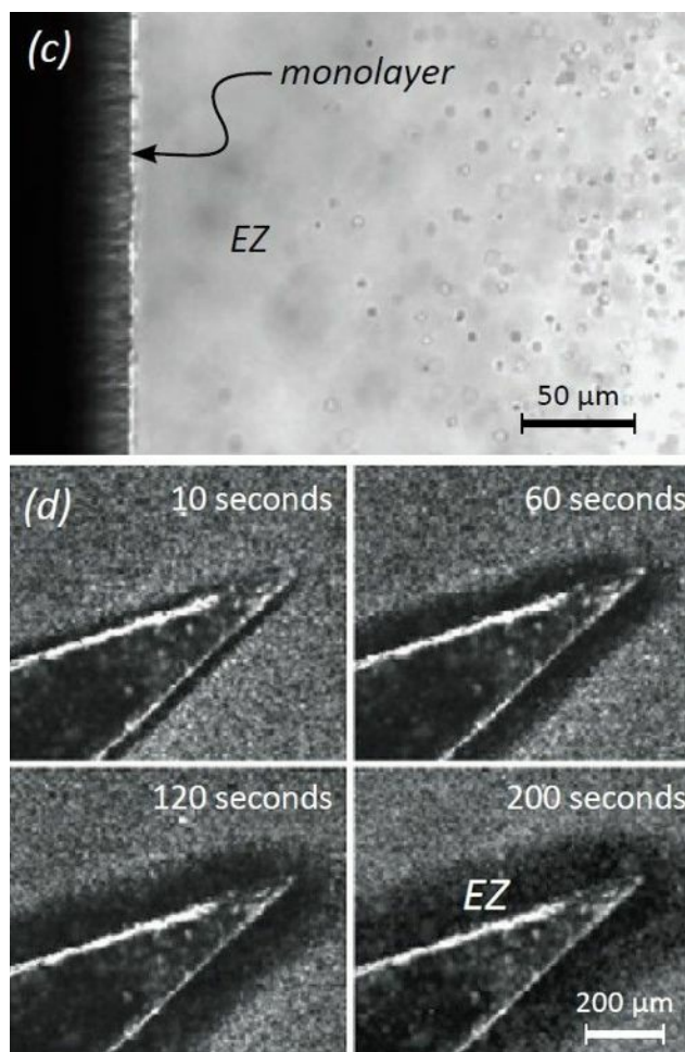
Fig. 3.9 Examples of microsphere-excluding zones, viewed in an optical microscope. (a) polyacrylic acid gel; (b) muscle; (c) a self-assembled monolayer on gold. (d) Nafion polymer, time series.
