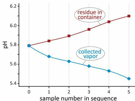
Fig. 14.5 Results of boiling experiments. Blue curve indicates pH of the vapor, collected after various durations of time. Red curve indicates pH of water remaining in the container following boiling.
