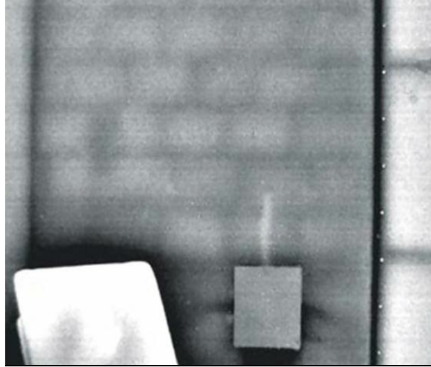
Fig. 10.5 Interior wall in a room situated just off a corridor. Observed with visible light (top) and with IR light (bottom). 1 The IR image reveals details of the wall's internal structure.
