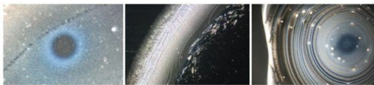
Fig. 13.8 Dried droplets, viewed in dark-field illumination. Left: spring water; middle: homeopathic preparation; right: dew droplet. Note blue color and concentric layering of shell.
