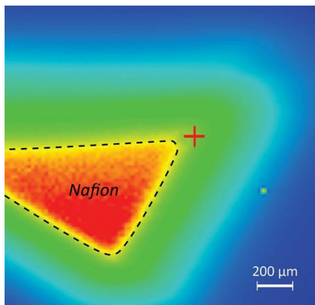
Fig. 3.14 Triangular specimen of Nafion in water examined using infrared absorption. Color differences indicate differences of absorption. Blue is lowest.
