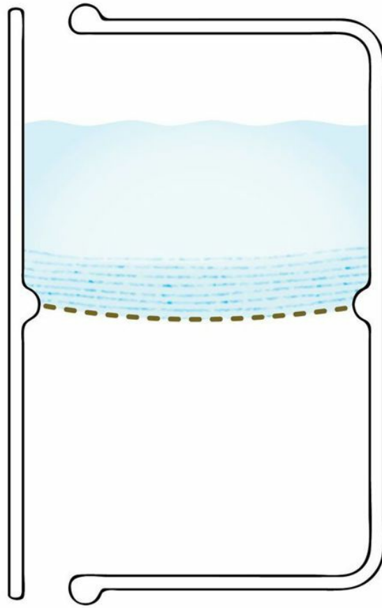
Fig. 11.6 Water fails to penetrate the EZ.
