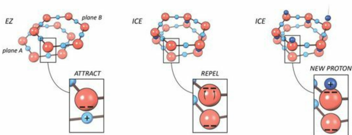
Fig. 17.13 Cooperative nature of ice formation. EZ configuration shown at left. In newly created ice layer (middle), oxygen's negative charge shifts upward (box), attracting incoming protons. This shift occurs in the three planar oxygen atoms juxtaposed to oxygen atoms beneath. Incoming protons settle at those three points (right), setting the stage for the next ice layer.
