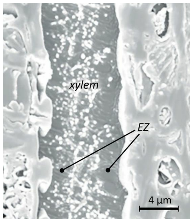
Fig. 16.15 Cryo scanning electron microscope image of ink particles infused into xylem. Particles concentrate in the center and are excluded from the zone near the walls. Courtesy Martin Canny.
