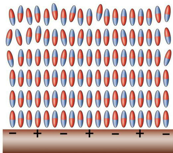
Fig. 4.4 Stacked dipole model of water ordering. Some loss of order might occur with increasing distance from the surface because of thermally induced motions.
