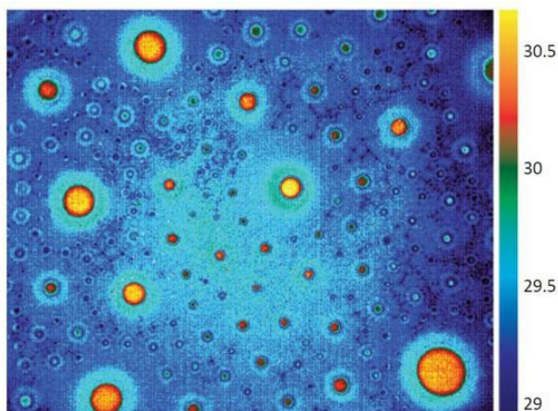
Fig. 14.6 Infrared image of surface bubbles. Bubbles were created by blowing air into a surfactant solution (TWEEN 20/water). Bubble interior (orange) generates more infrared energy than the exterior (blue). Darkness of thin bubble boundaries is expected — EZs generate little infrared energy. Scale in °C.
