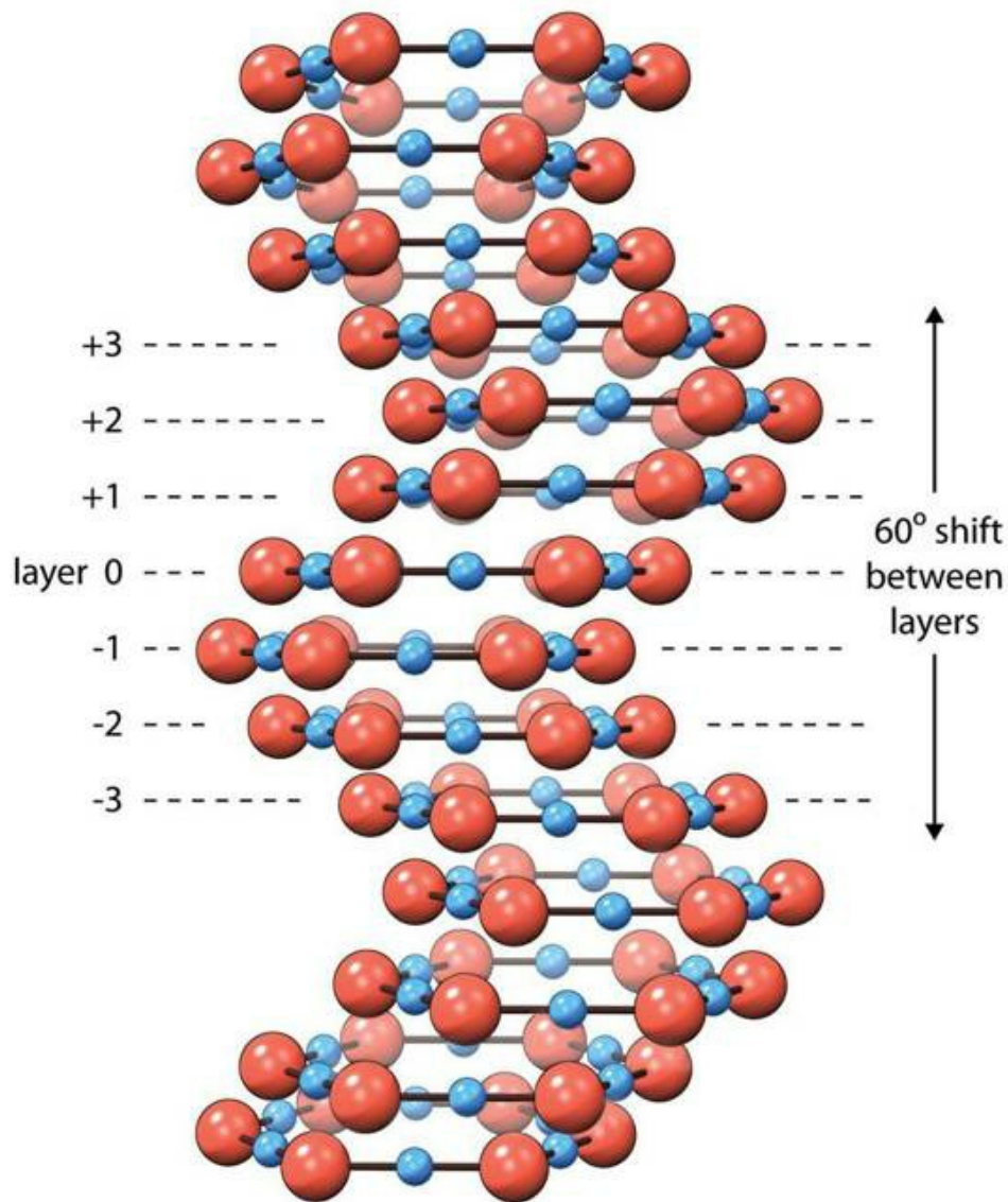
Fig. 4.14 Shifting successive planes by 60° yields a helical structure.
