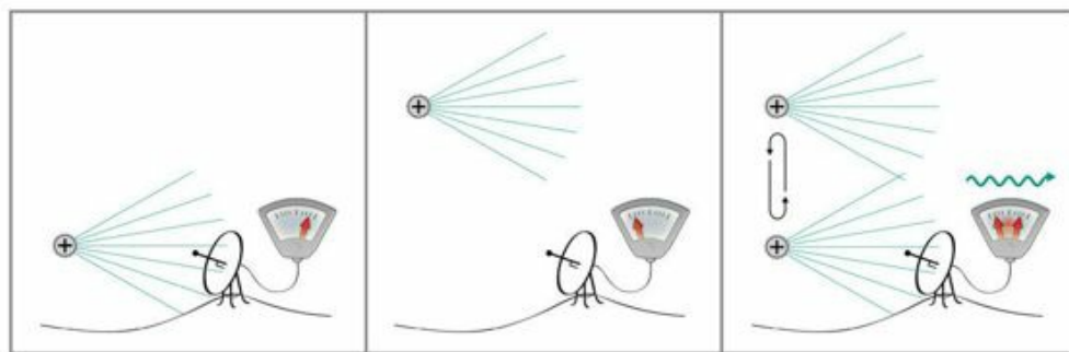
Fig. 10.3 Electromagnetic wave generation (simplified). Back-and-forth movement of the charge creates an oscillating electric field, which a sensor can pick up.
