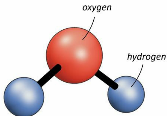
Fig. 2.1 Artist's sketch of the water molecule.
