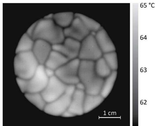
Fig. 15.3 Infrared image of a dish of warm water, taken from above. Equivalent temperature scale at right.
