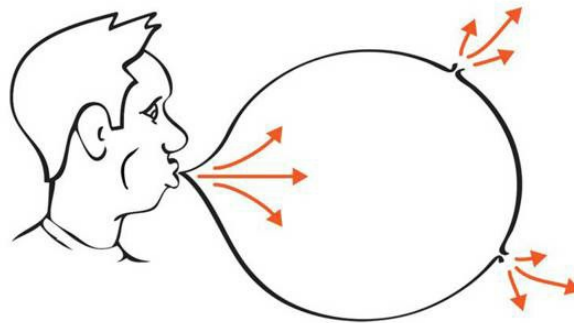
Fig. 7.4 Relief valve. A continuous release of energy assures that the system never overloads and explodes.
