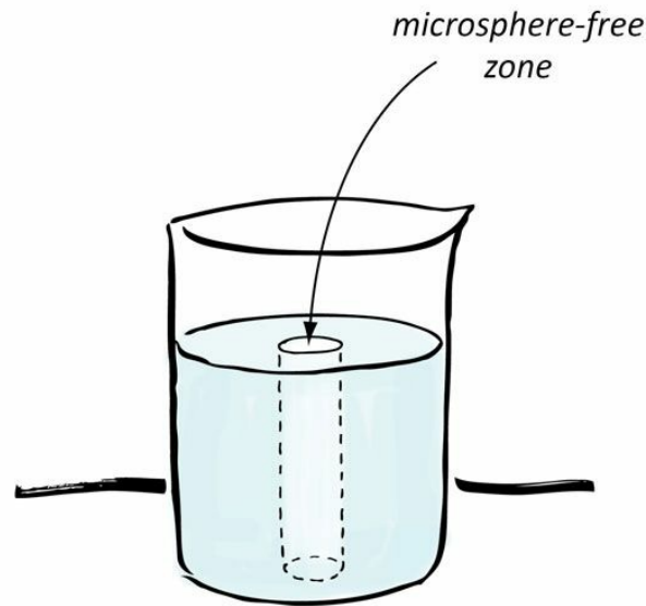
Fig. 1.3 Near-central clear zone in microsphere suspension. Why does the microsphere-free cylinder appear spontaneously?
