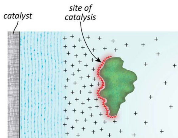
Fig. 12.11 EZ-based catalysis. The catalyst surface nucleates EZ growth, which results in proton (or \text{OH}^- ) release. The protons (or \text{OH}^- groups) accelerate the target reaction.
