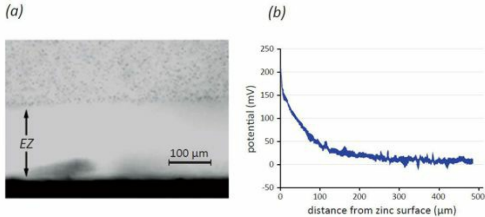
Fig. 12.9 Zinc-surface features. 4 (a) Exclusion zone found next to zinc. (b) Electrical potential within the EZ
