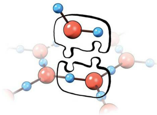
Fig. 6.13 Adding elements to the lattice.
