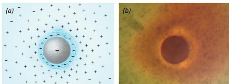
Fig. 8.9 Spherical particles immersed in water. (a) Diagram showing surrounding charges. (b) Negatively charged bead (dark) immersed in water with pH dye. Lighter region around the dark sphere is the EZ, which excludes pH dye. Intensely red region beyond indicates low pH, or high concentration of protons.
