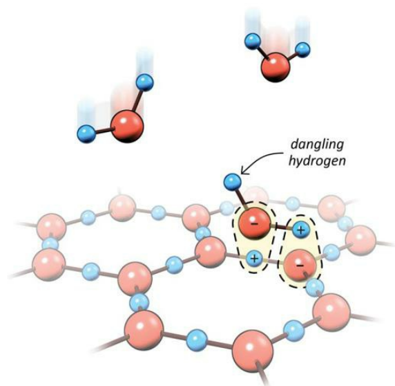
Fig. 6.7 Building the exclusion zone. Freed water molecules draw toward the exposed EZ layer because EZ surface charges attract opposite charges on the water molecule. Following attachment, a hydrogen atom dangles.
