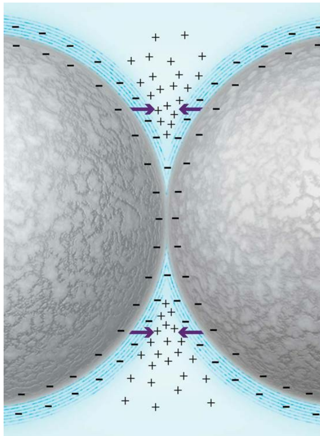
Fig. 8.12 Stable points for smaller (top) and larger particles (bottom). End points occur when attractions balance repulsions.
