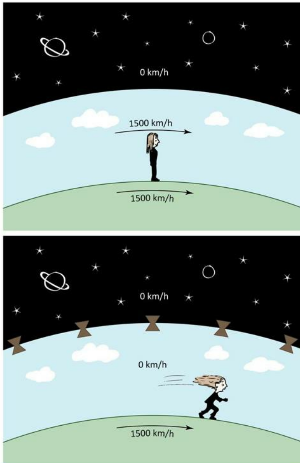
Fig. 15.19 Earth-atmosphere coupling. The atmosphere moves together with the earth's surface (top). In the absence of coupling between air molecules, the atmosphere might not move much at all (bottom). An earthbound observer would then detect an east-to-west wind of high velocity all the time.
