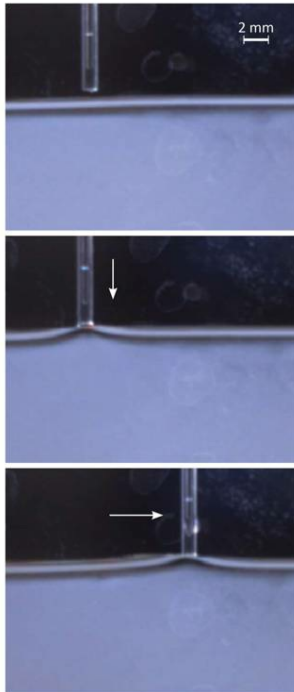
Fig. 16.3 Glass probe lowered to touch the top surface of water. Thickness of EZ is hardly altered by that mechanical perturbation or by
