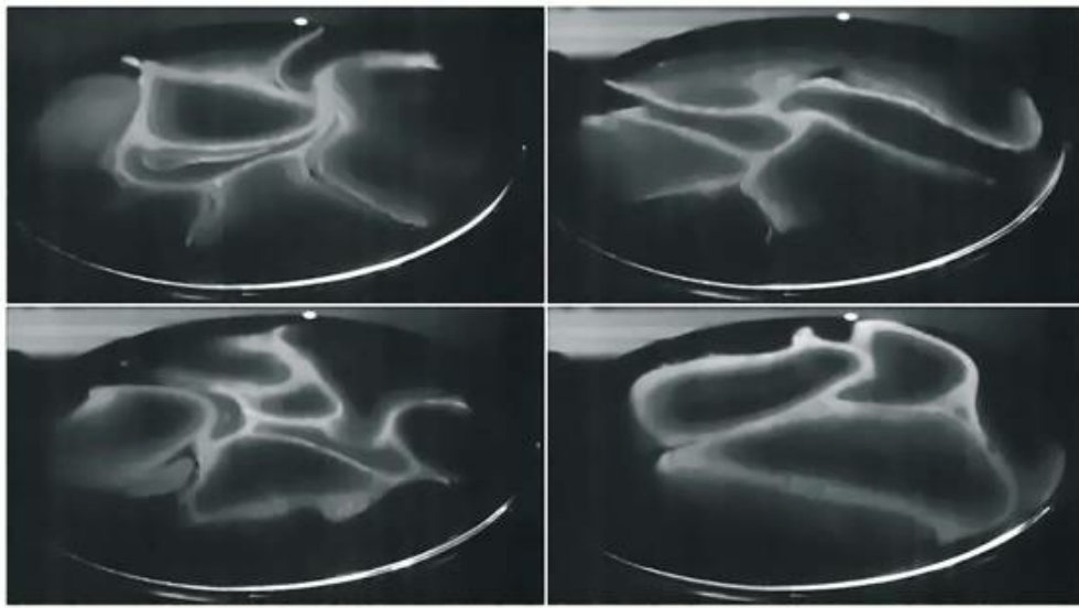
Fig. 15.2 Examples of vapor rising from warm water. The white rings represent high concentrations of vesicles, which form the visible vapor.
