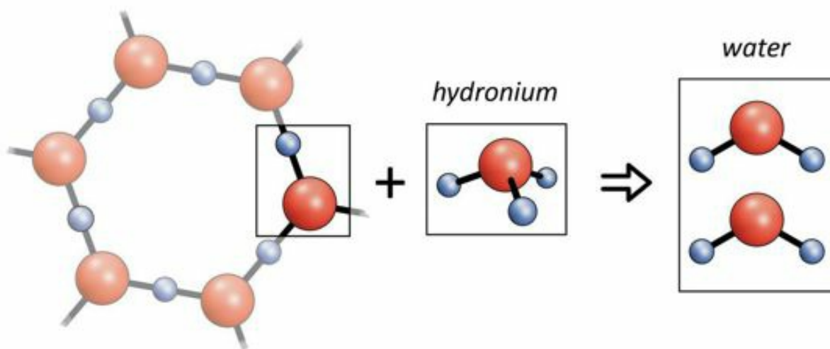
Fig. 6.11 Natural erosion of exclusion zone. Combining a hydronium ion with one EZ structural unit extracts that unit from the lattice, resulting in two water molecules.
