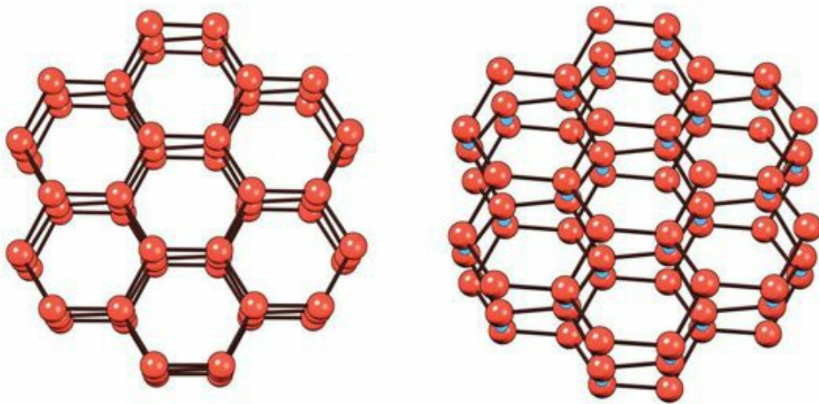
Fig. 4.5 Structural model of common ice viewed from two different angles. Oxygen atoms are red. Hydrogen atoms (not shown) lie midway along the lines connecting the oxygen atoms. Interplanar protons (blue, bottom) link every other oxygen. The linkages create a pucker, which makes the arrangement of atoms seem less planar and more tetrahedral.
