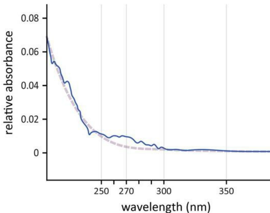
Fig. 10.11 Spectral measurements of vortexed water. Preliminary observations show EZ growth.
