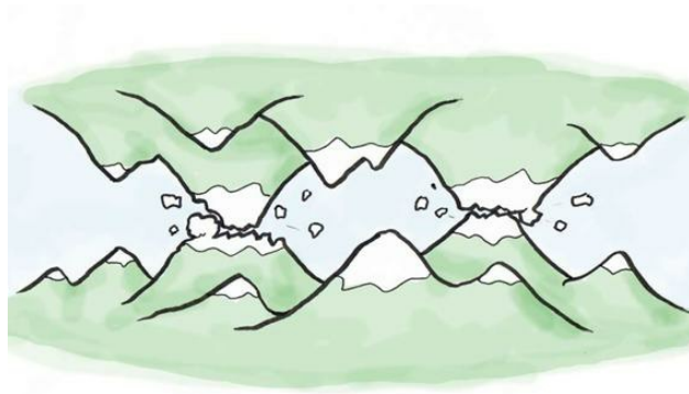
Fig. 12.1 Friction analogy. When the upper “mountain range” slides past the lower one, the resistance creates friction.
