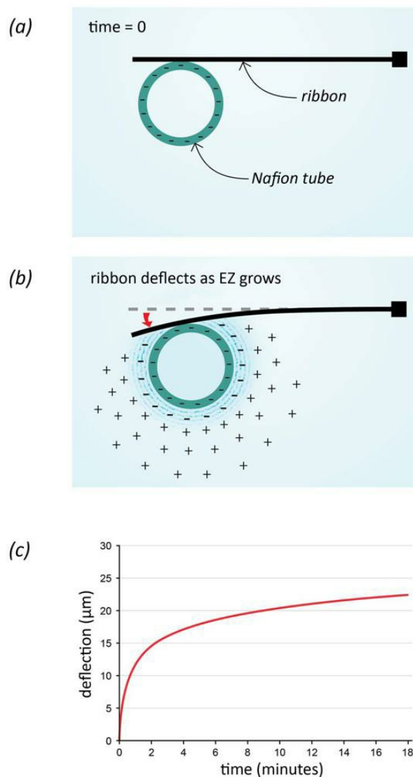
Fig. 9.9 EZ deflection toward protons. (a) Nafion tube mounted on ribbon face; (b) ribbon deflecting toward protons; (c) measured time course of deflection.
