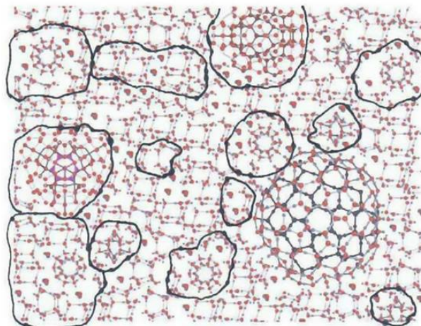
Fig. 2.3 Proposed structure of liquid water, from Rustum Roy and colleagues. 3 Clusters are outlined in black.
