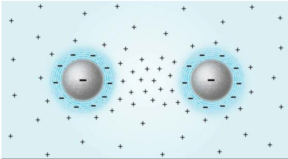
Fig. 8.10 Expected distribution of charge when two spheres lie near one another. The positives in the middle do not significantly disperse because of their attraction to EZ negativity.
