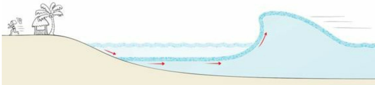
Fig. 16.6 Tsunami dynamics with an elastic surface sheet. An upswell will draw the elastic sheet seaward, as observed.
