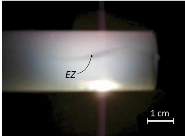
Fig. 9.13 Light-induced deflection of microsphere-free zone. This EZ projects from a nucleating surface positioned off to the left. The light beam projects from bottom to top. Microspheres drawn toward the light cause the EZ to shift oppositely.
