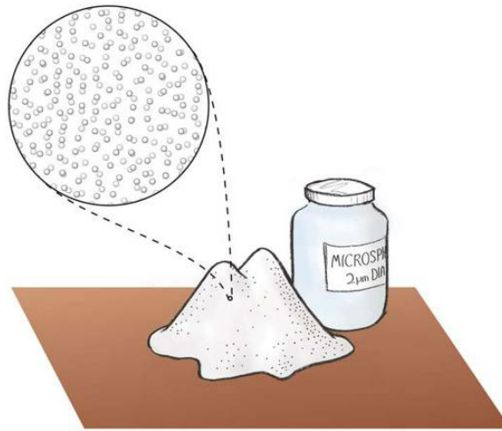
Fig. 3.1 Microspheres are common tools for scientists.
