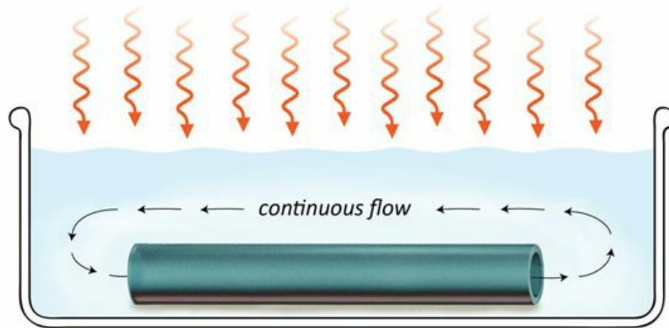
Fig. 12.13 “Spontaneous” flow through hydrophilic tubes.
