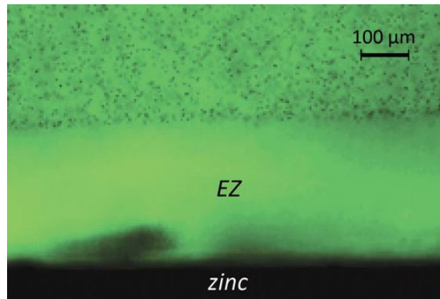
Fig. 3.6 Exclusion zone next to zinc, from reference 5. Green color results from using a green filter in the microscope.
