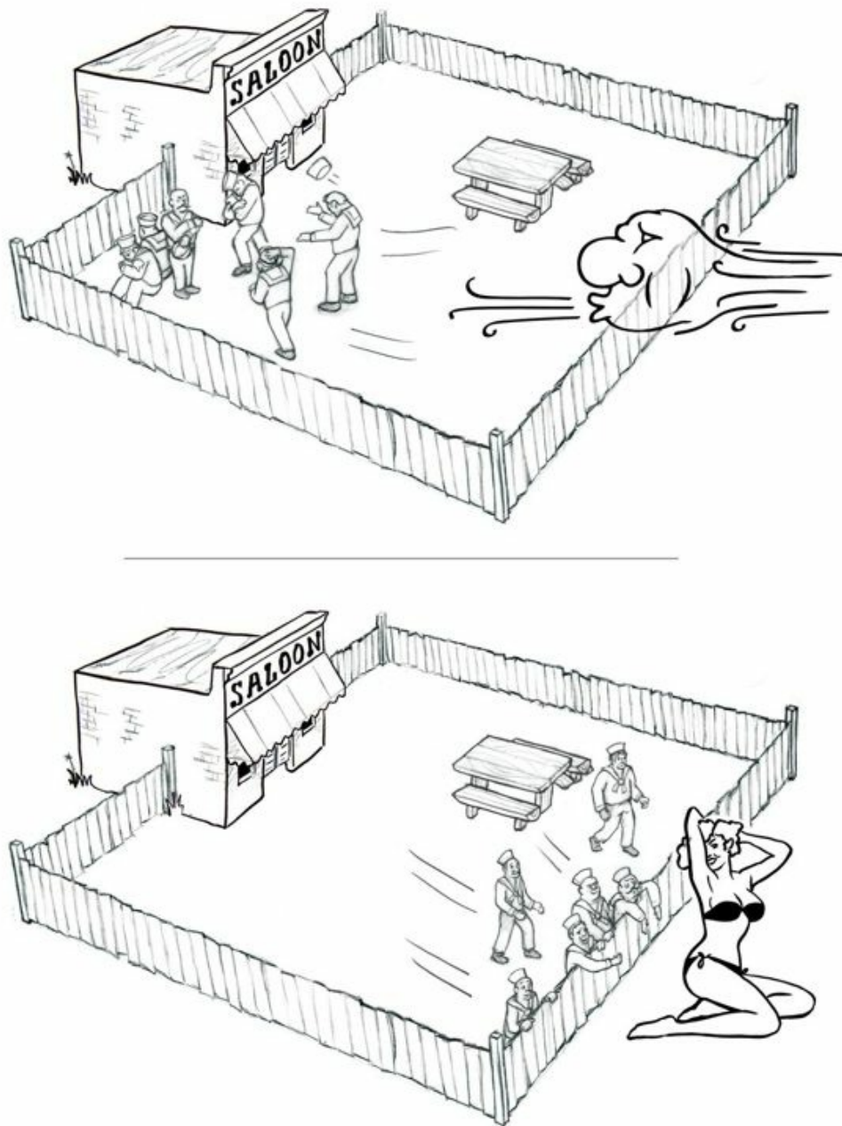
Fig. 11.3 Diffusion analogy. Diffusive movements are driven by external energy (top) and subject to agents of distraction (bottom).
