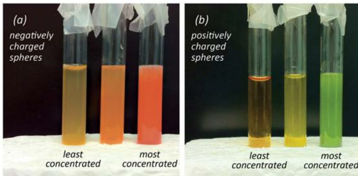
Fig. 5.5 Addition of microspheres alters water's pH. (a) Carboxylate microspheres, 1 \mu\text{m} diameter. Increasing microsphere concentration changes dye color toward red, indicating lower pH. (b) Positively charged amino microspheres change dye color toward green, indicating higher pH.
