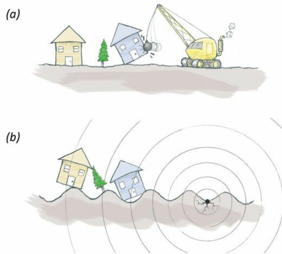
Fig. 9.16 (a) Einstein's formulation emphasizes local influence. (b) The EZ formulation implies long-range influence.
