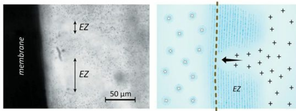
Fig. 11.7 EZ breaches observed microscopically (left). To create the breaches, positive charges invade the negatively charged EZ, eroding it locally (right).
