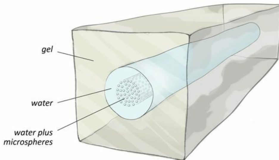
Fig. 3.2 Schematic diagram illustrating the microsphere-free zone just inside the gel tunnel.
