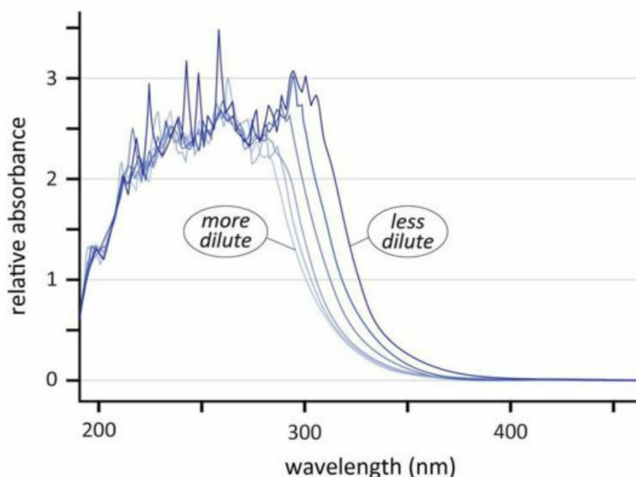
Fig. 10.10 Ammonium persulfate dissolved in water. With increasing dilution (right to left), the area beneath the absorption peak diminishes.
