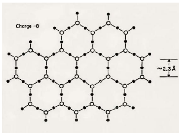
Fig. 4.9 Molecular structure of polywater, proposed by Lippincott and colleagues. 6 Oxygen molecules denoted by open circles, hydrogens solid. Sheets stack to yield volumetric structure.
