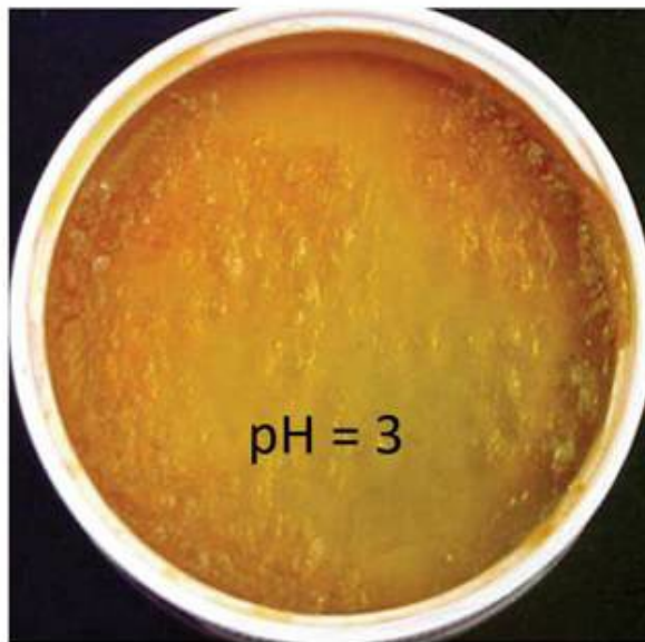
Fig. 17.7 Water containing diluted pH dye. pH values refer to the chambers' peripheries.
