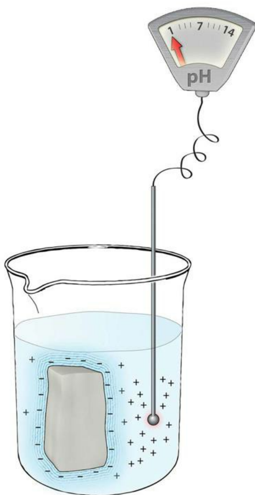
Fig. 4.8 Measuring the pH of water next to an
