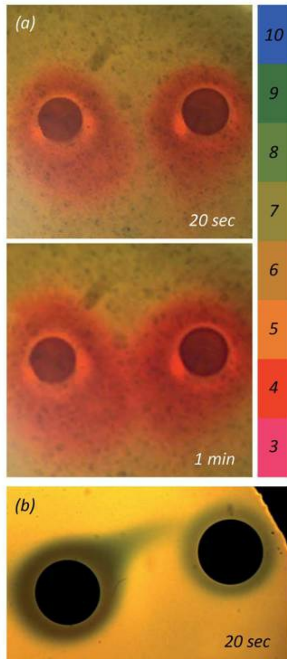
Fig. 8.11 Unlike charges situated between like-charged spheres. (a) Dye shows region of low pH (numerous protons or hydronium ions) in between two negatively charged beads. At right, pH scale. (b) Region of high pH (negative charges) lying between two positively charged beads. Negative charges sometimes coalesced
