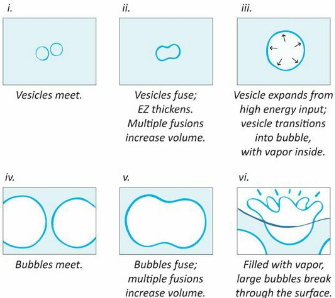
Fig. 14.12 The processes leading to boiling during high radiant energy input.
