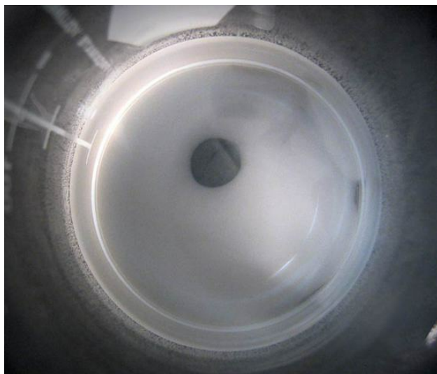
Fig. 9.12 Microsphere-free zone in a beaker (viewed from above). Running from top to bottom, the clear zone appears near the center of the aqueous microsphere suspension.
