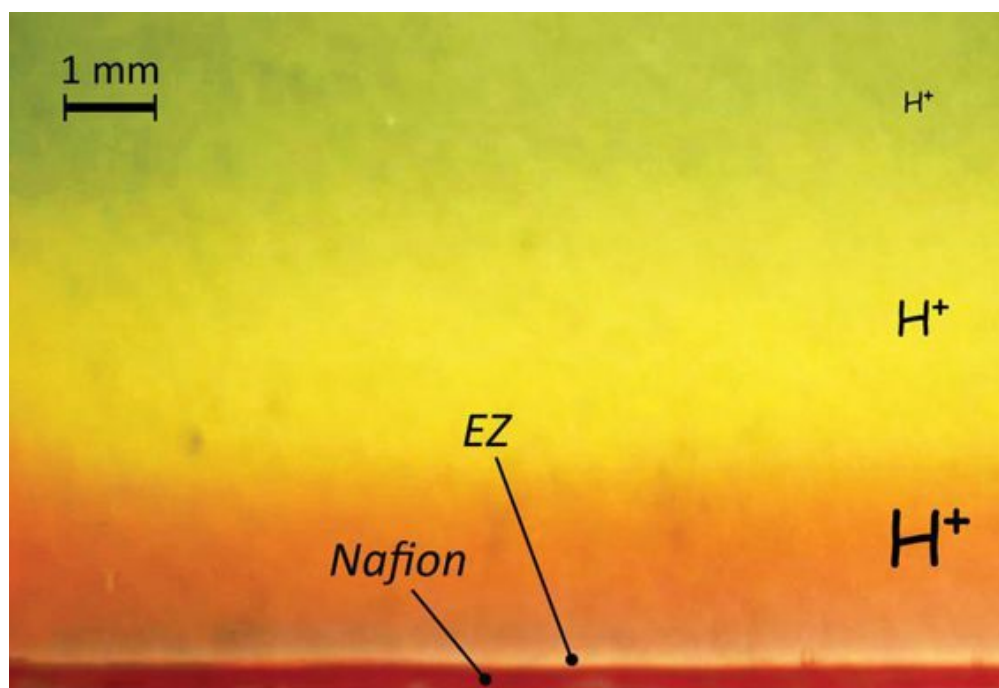
Fig. 5.3 Proton distribution beyond the exclusion zone (viewing the wide face of a narrow chamber). This image, obtained shortly after pouring water with
