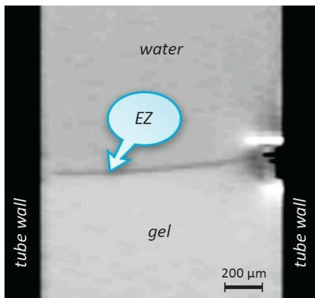
Fig. 3.16 MRI map of relaxation times. The lower half of a capillary tube was filled with polyvinyl alcohol gel, while the upper half was filled with water. The dark band, corresponding to the gel's EZ, indicates more molecular restriction.
